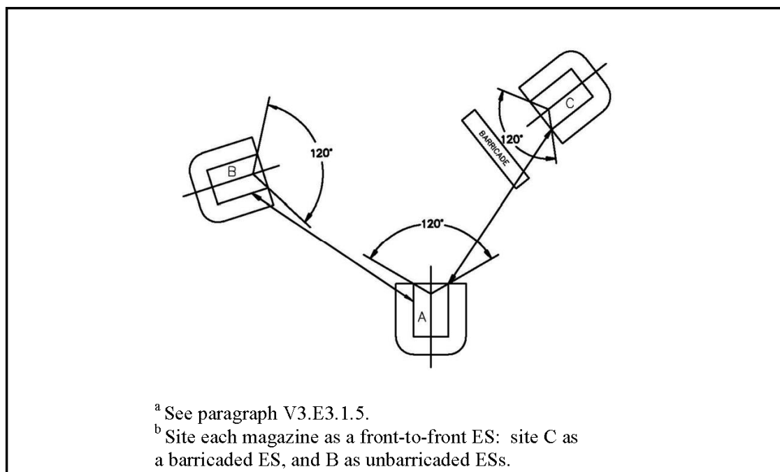
Figure V3.E3.F6. ECM Orientation Effects on IMD: Canted ECMs a, b, c
