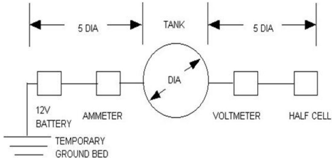
Figure A7.2. Measuring Resistance to Earth of Large POL Tank.
