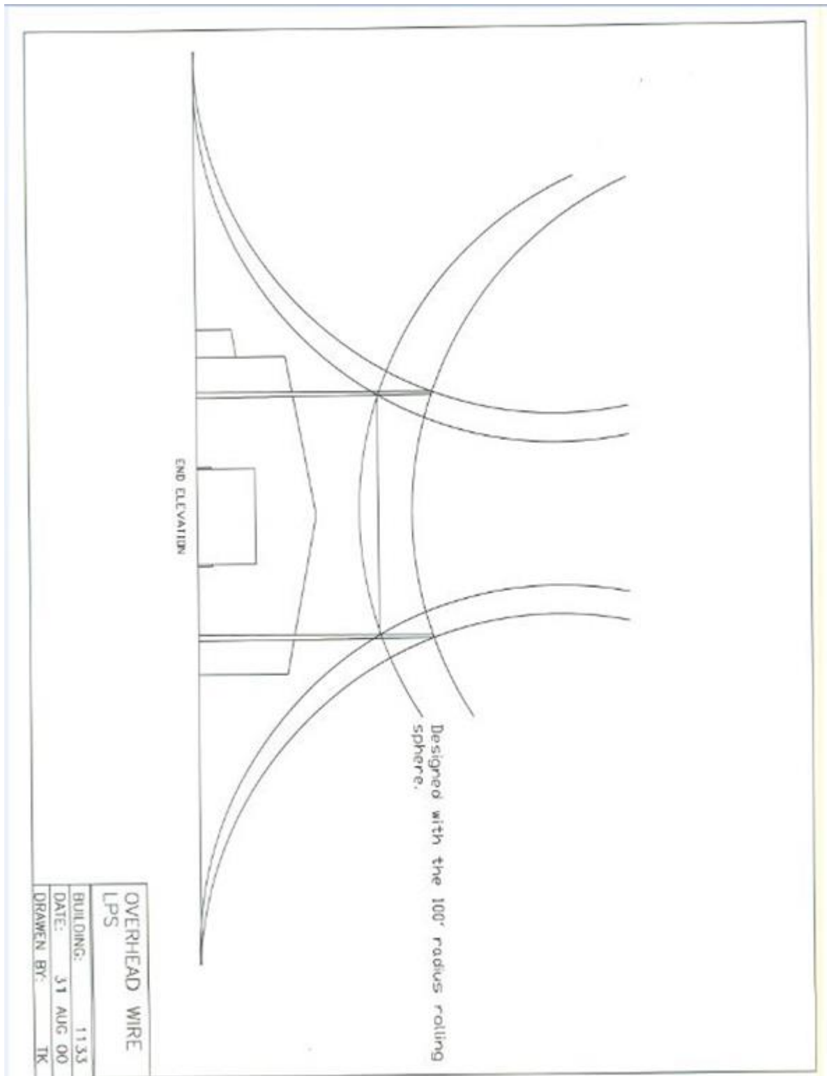
Figure A7.10. Sample Record for Projected Rolling Sphere Protection (100' is for Explosives Facilities – Non-explosives Facilities may be 150').
