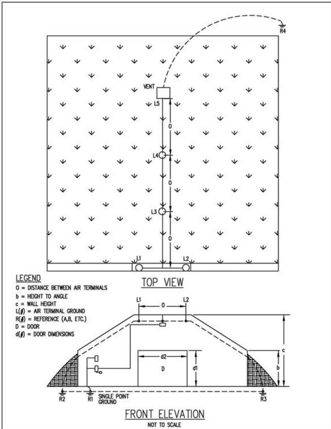
Figure 12.1. ECM With Center Conductor and Air Terminals.
