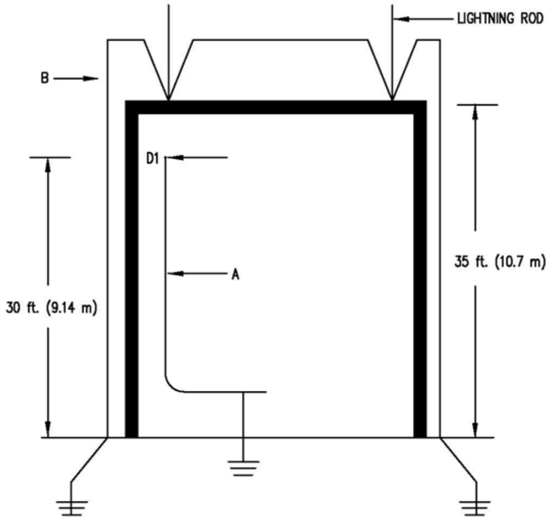
Figure A4.4. Typical Bonding Conditions in Structures 40 Feet or Less in Height.
