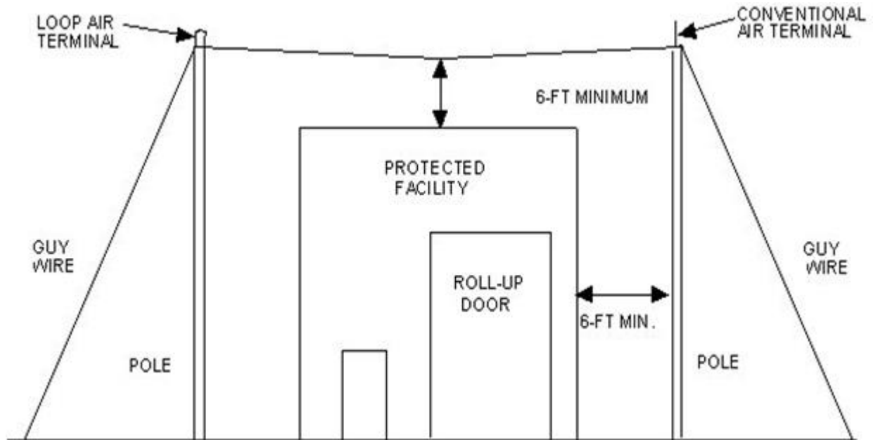
Figure A5.1. Air Terminals on Masts (Typical).
