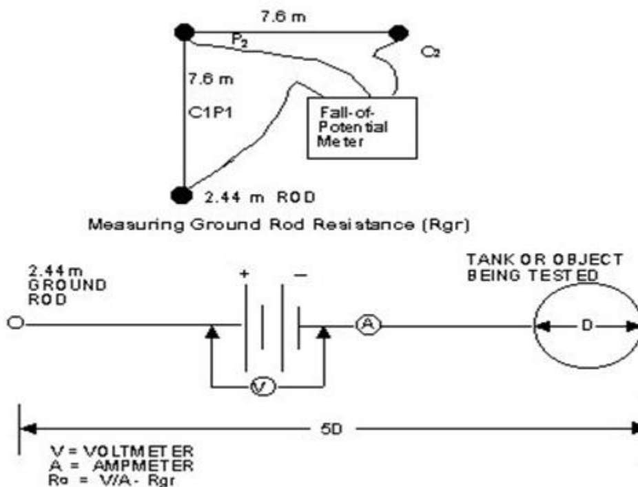
Figure A7.3. Alternate Method of Measuring Resistance to Earth of Large Object.
