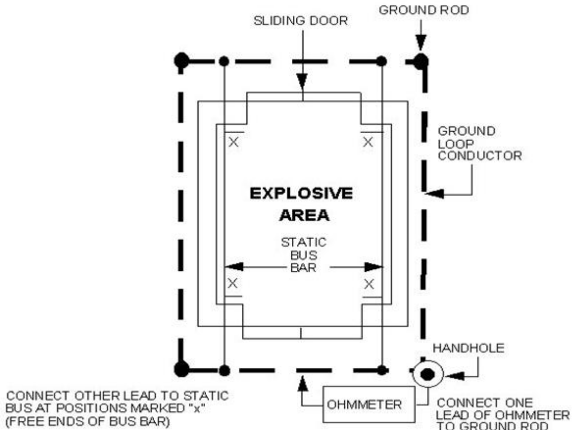
Figure A7.5. Testing Static Bus Bars in Typical Explosives Area.
