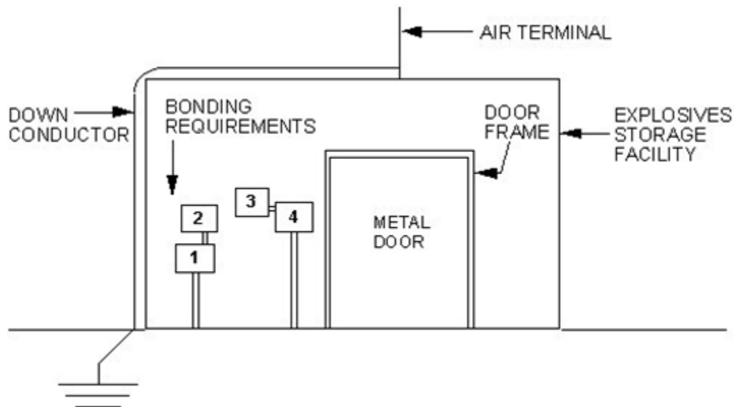
Figure A4.9. Bonding for Typical Air Force Structure.
