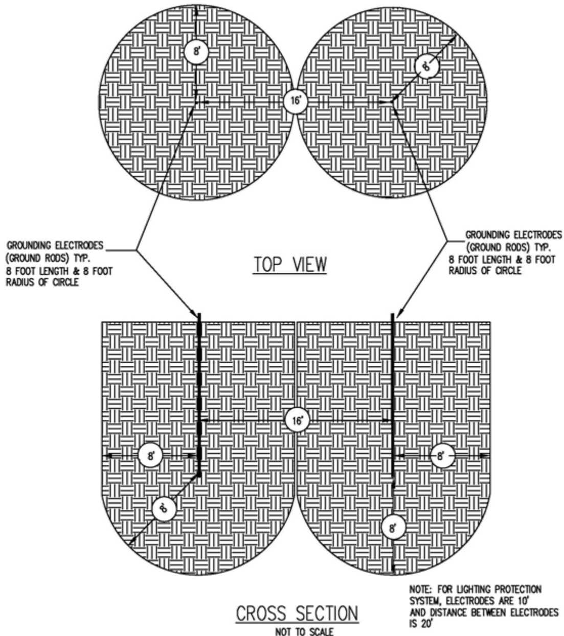
Figure A3.2. Parallel Grounding Electrodes at Service Entrances (Also See NEC Minimums).
