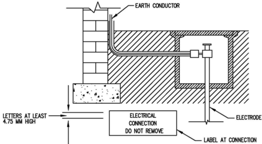
Figure A3.1. Test Well Configuration Example.
