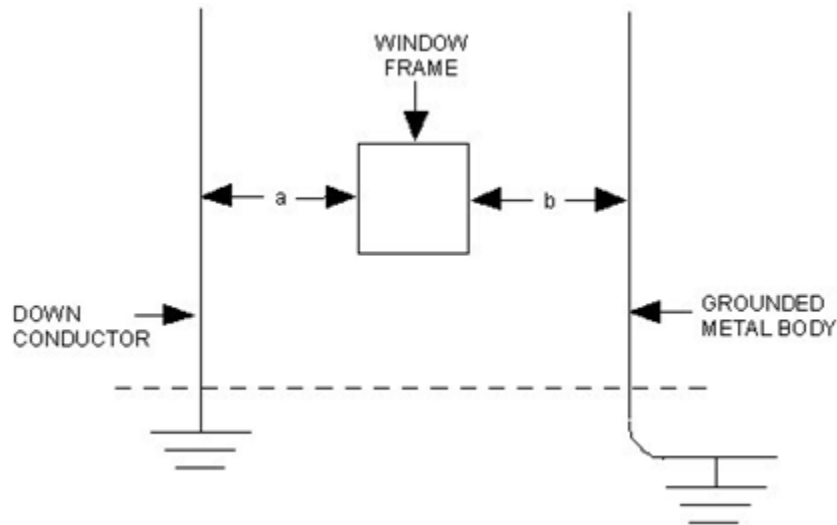
Figure A4.6. Typical Bonding Conditions for Ungrounded Metal Bodies.
