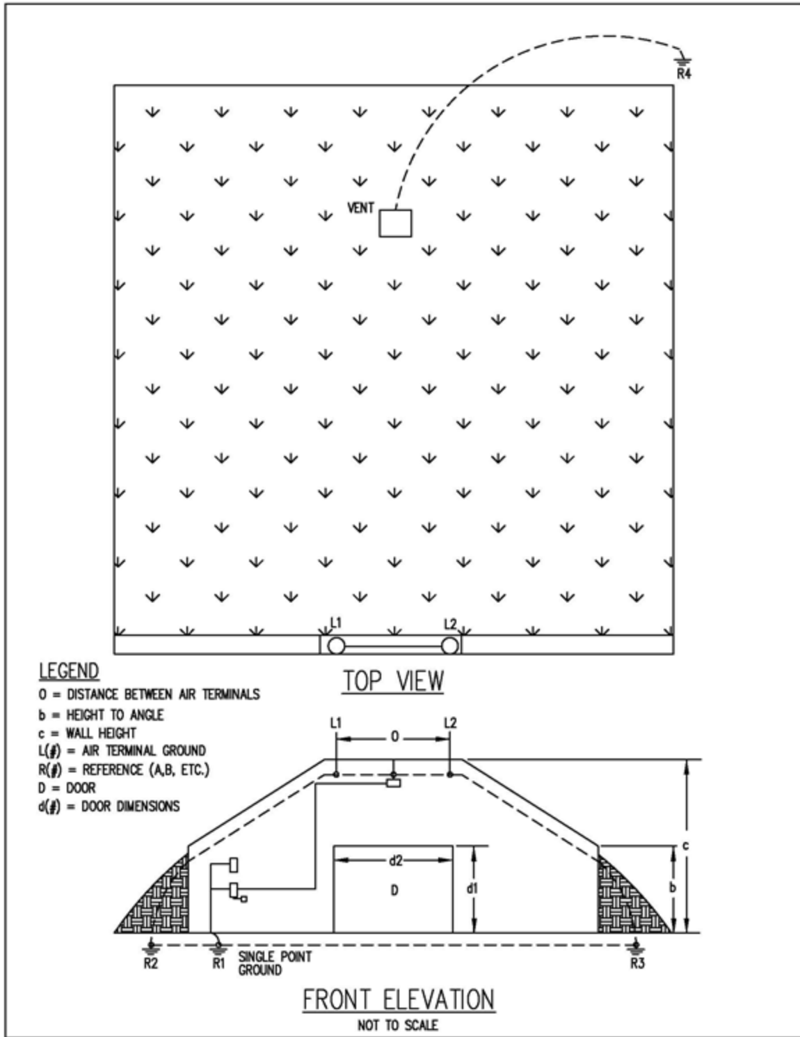
Figure 12.2. ECM Without Center Conductor and Air Terminals.
