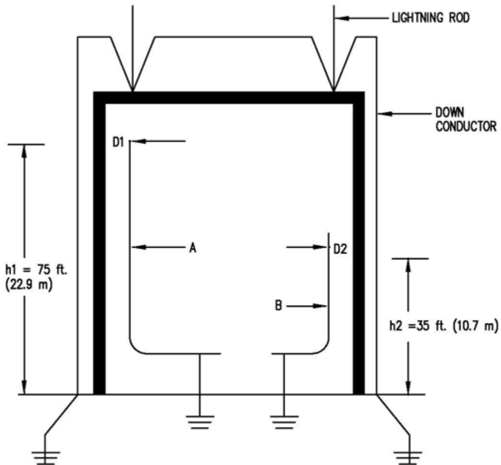
Figure A4.5. Typical Bonding Conditions in Structures Greater Than 40 Feet in height. [D 2 cut off]
