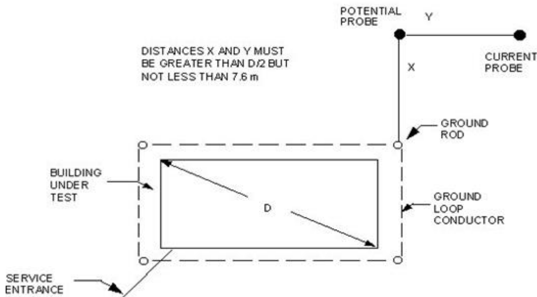
Figure A7.1. Auxiliary Probe Locations for Fall-of-Potential Ground Resistance Test.
