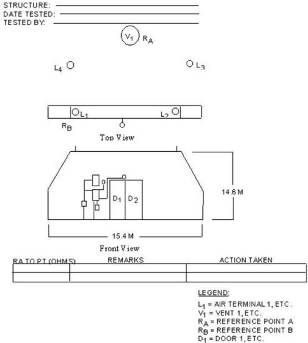
Figure 10.1. Example Sketch of Test Points (Typical).
