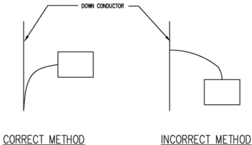
Figure A4.7. Bonding Metallic Equipment to Down Conductor.
