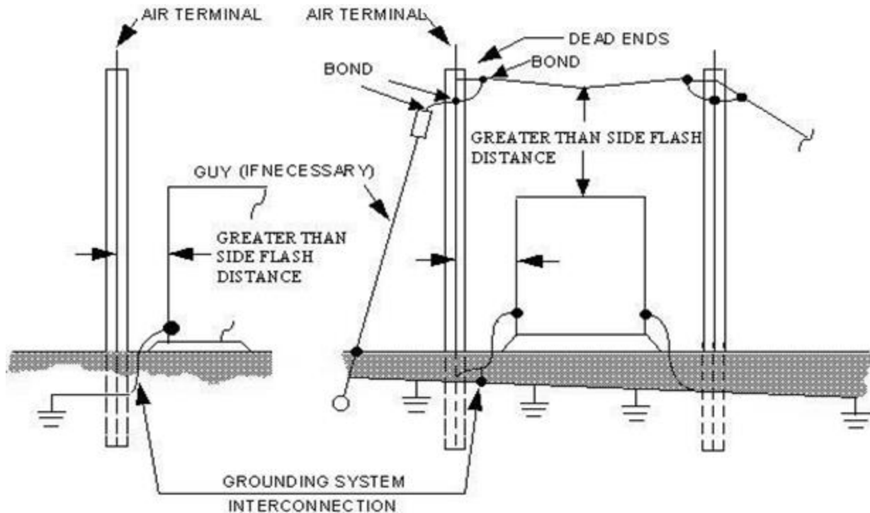
Figure A7.4. Mast System (a) and Overhead Wire or Catenary System (b).
