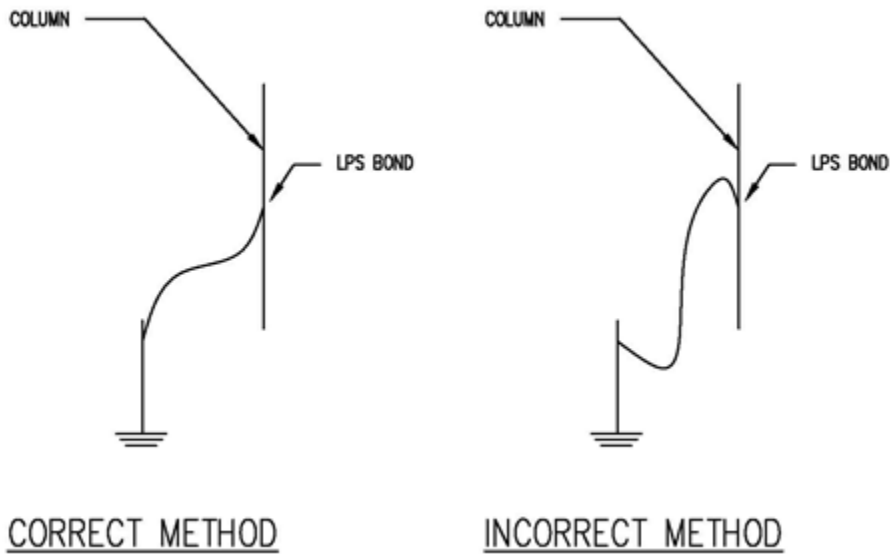
Figure A4.8. Bonding Down Conductor to Grounding Electrode.
