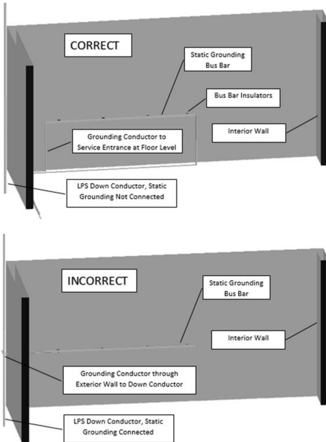
Figure 11.1. Grounding Static Bus Bar on Interior Wall.
