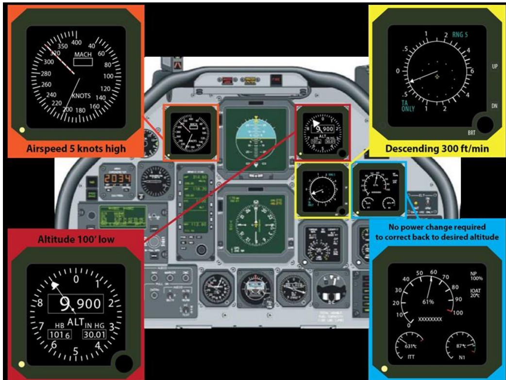
Figure A5.3. Airspeed Deviation.
