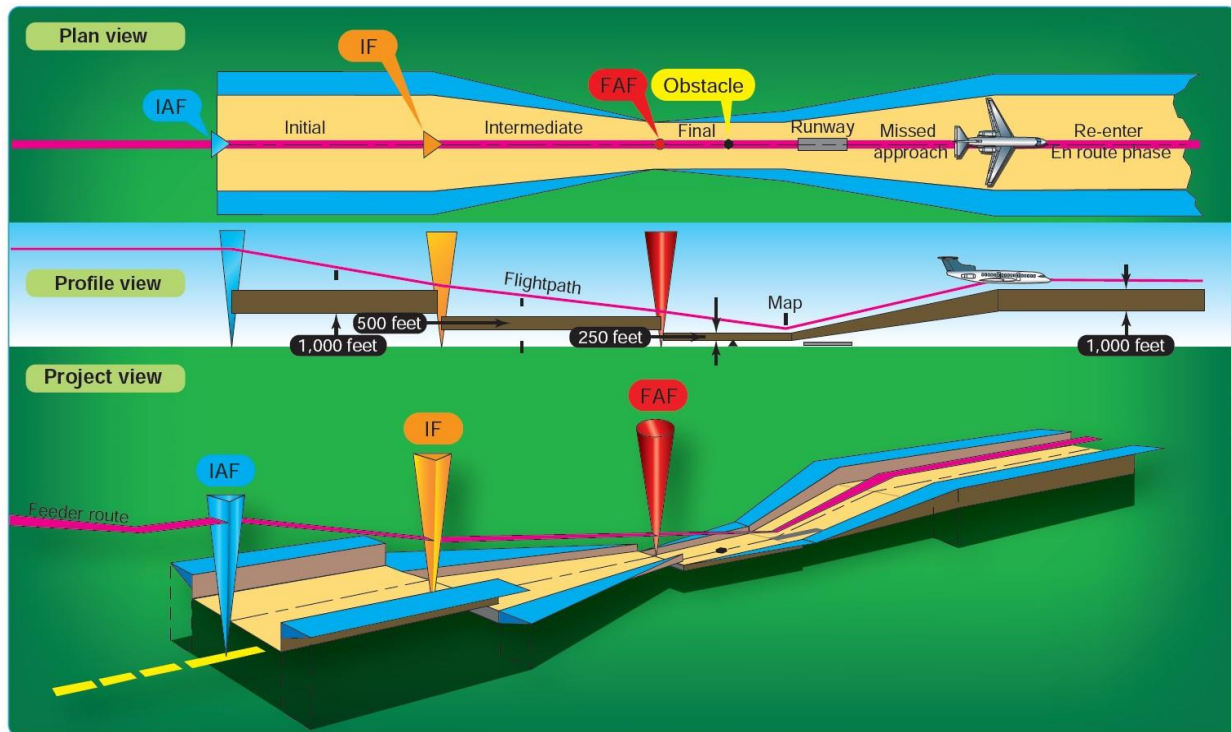
Figure 15.10. Approach Segments.
