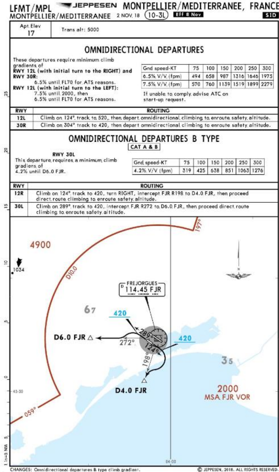
Figure 5.6. Omnidirectional Departure.
