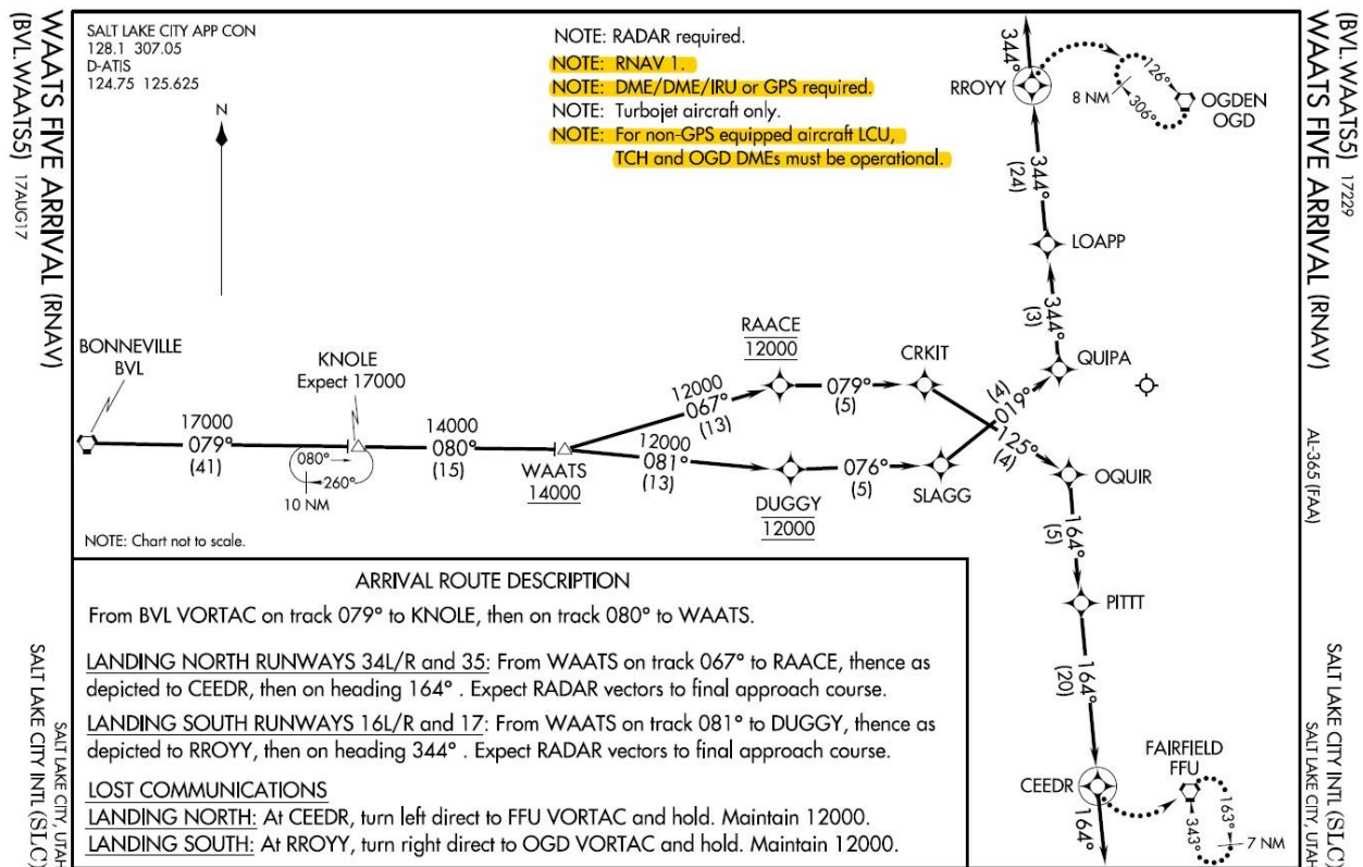
Figure 14.1. RNAV Arrival.
