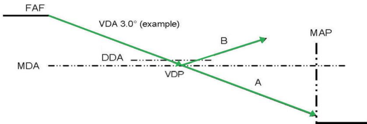
Figure 16.5. CDFFA.
