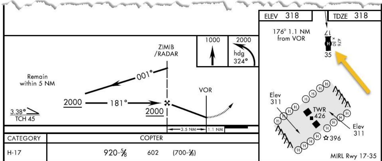
Figure 15.30. Helicopter-Only Approach.
