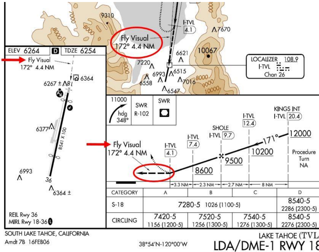
Figure 16.10. Visual Segment.
