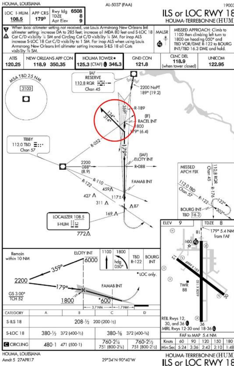
Figure 15.17. Procedure Turn.
