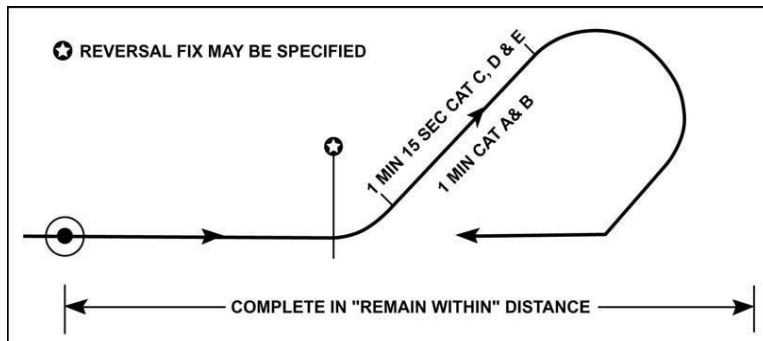
Figure 15.21. 45°/180° Procedure Turn.
