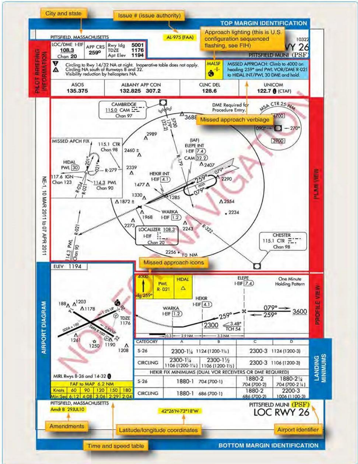
Figure 15.4. Instrument Approach Chart.
