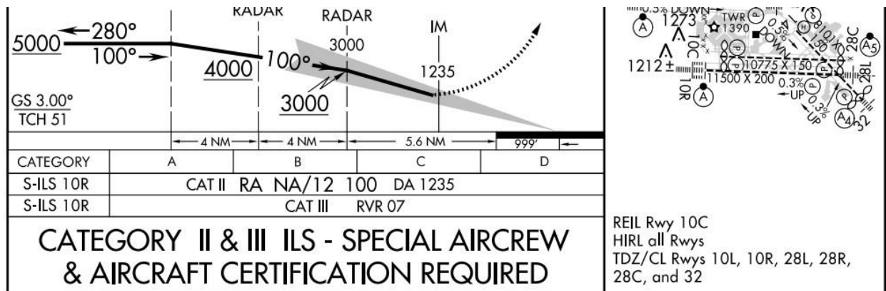
Figure 17.2. CAT II ILS Approach.
