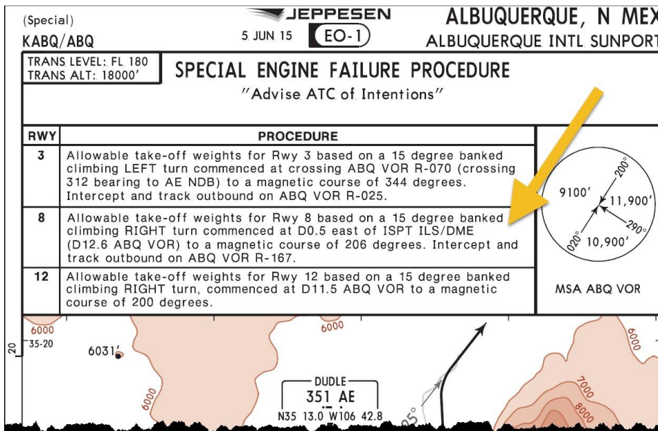
Figure 5.24. Albuquerque SDP (Runway 8).
