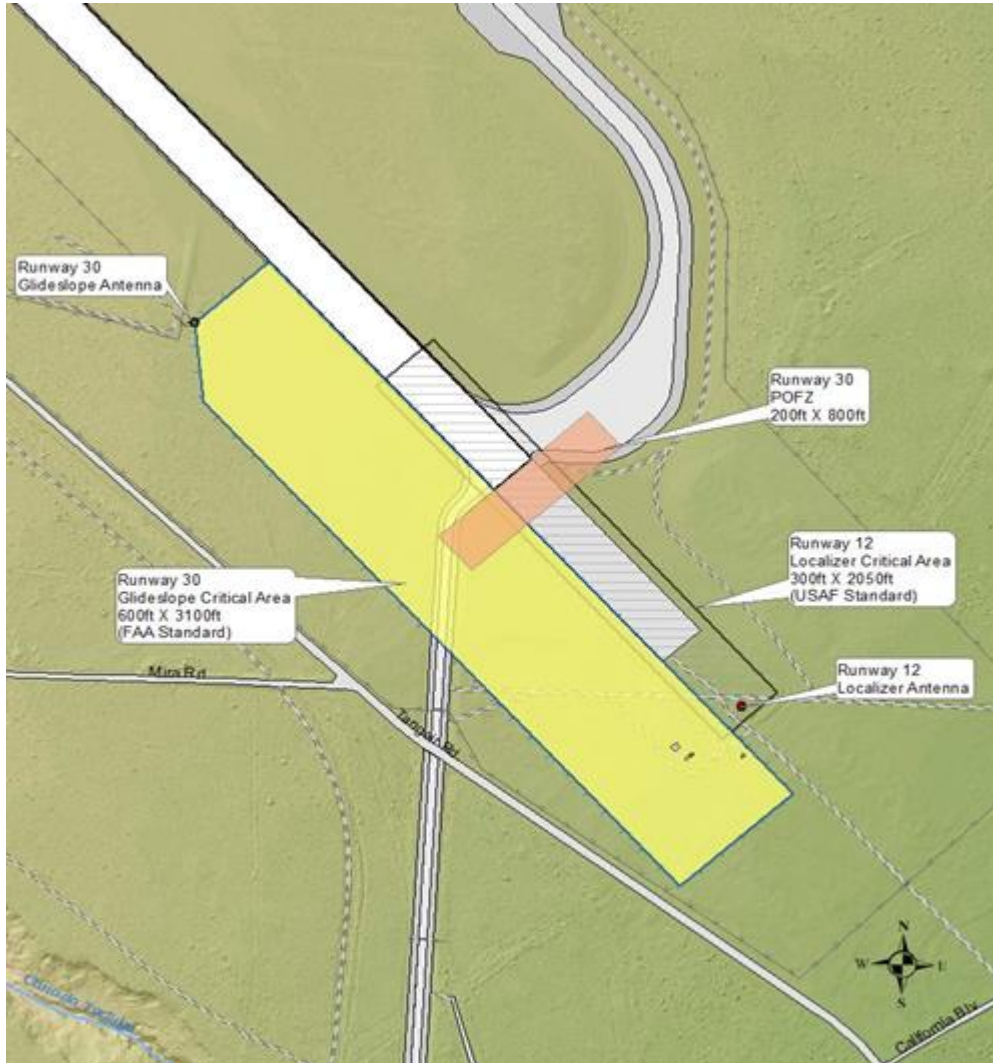
Figure A13.1. (Added-SLD30) Runway 30 Glideslope Critical Area, Runway 12 Localizer Critical Area and Runway 30 POFZ.
