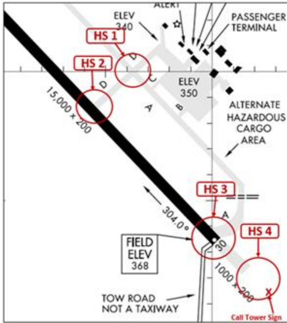
Figure 4.1. (SLD30) Hot Spots.
