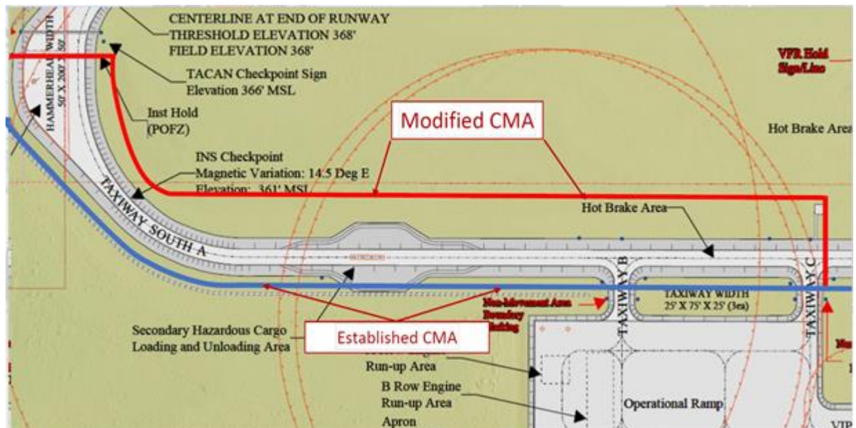
Figure 4.3. (Added-SLD30) Taxiway South Alpha CMA Modification.
