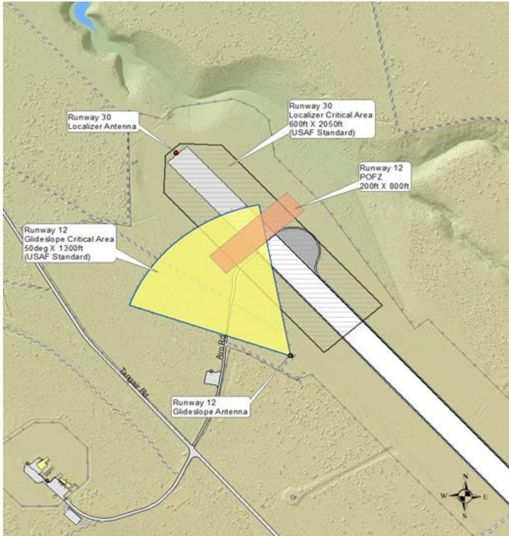
Figure A12.1. (Added-SLD30) Runway 30 Localizer Critical Area, Runway 12 Glideslope Critical Area and Runway 12 POFZ.
