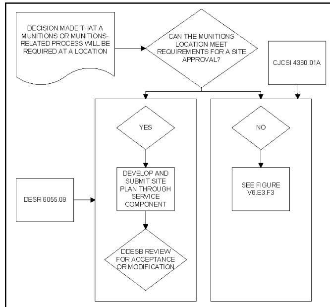
Figure V6.E3.F2. Explosives Safety Site Planning Process Decision Matrix (Locations That Can Meet Requirements)
