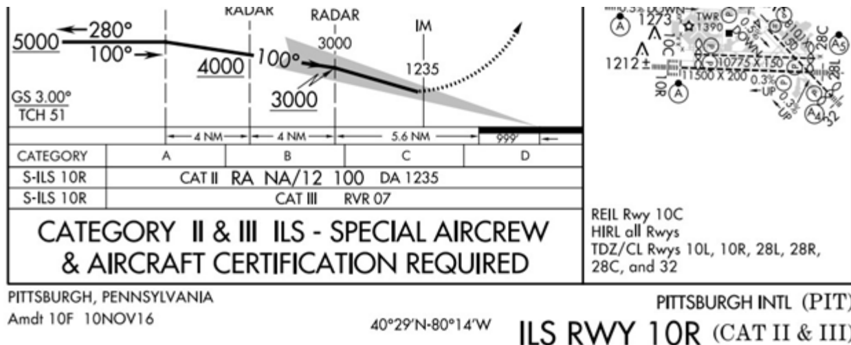
Figure 17.2. CAT II ILS Approach.
