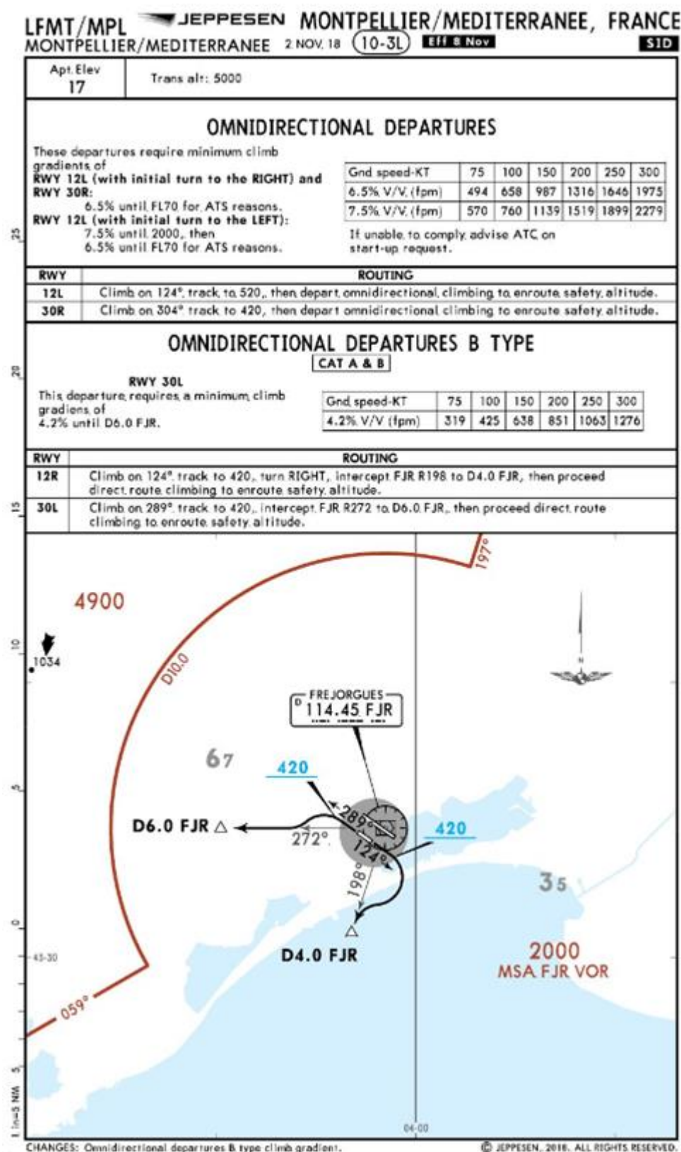
Figure 5.6. Omnidirectional Departure.
