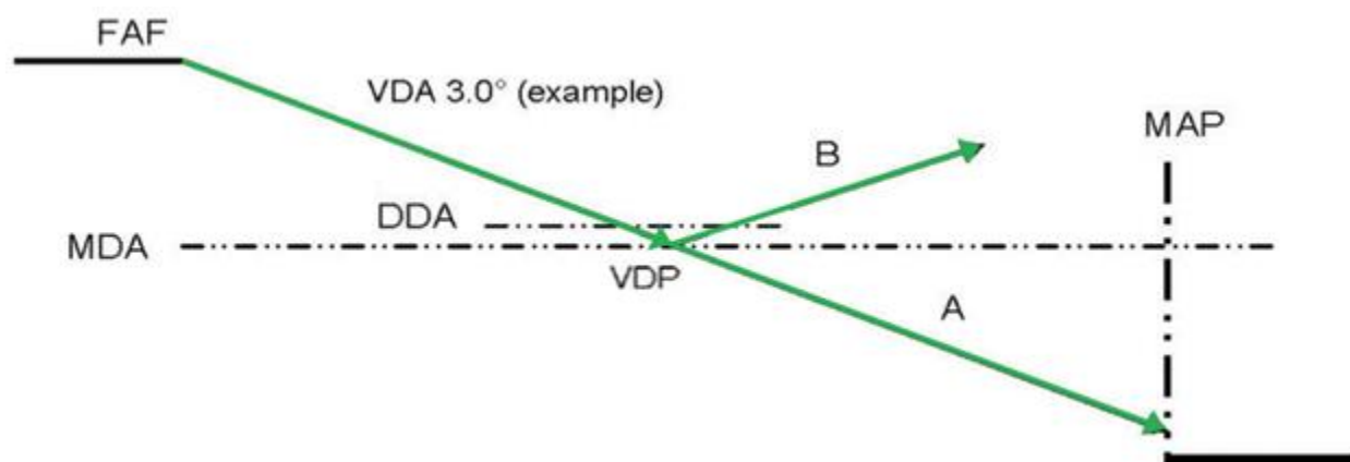
Figure 16.5. CDFA.
