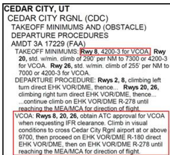
Figure 5.13. VCOA Format.
