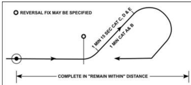
Figure 15.21. 45°/180° Procedure Turn.
