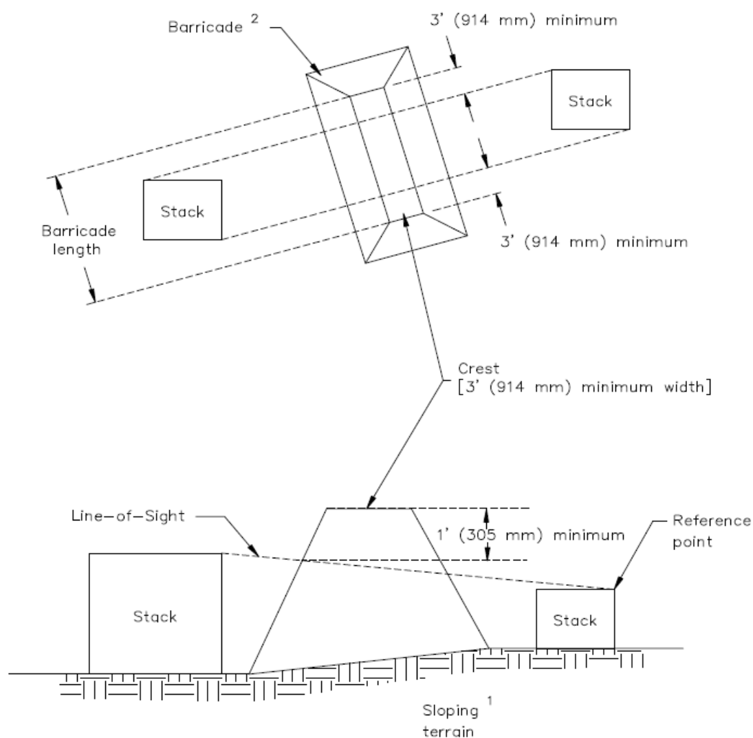
Figure 6.2. Determination of Barricade Length and Height to Prevent Prompt Propagation Due to High-Velocity, Low-Angle Fragments.
