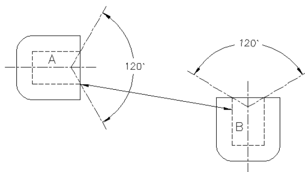
Fig122A ECM Orientation Effects on IMD: Side-to-Side Orientation (see paragraph 1225)
