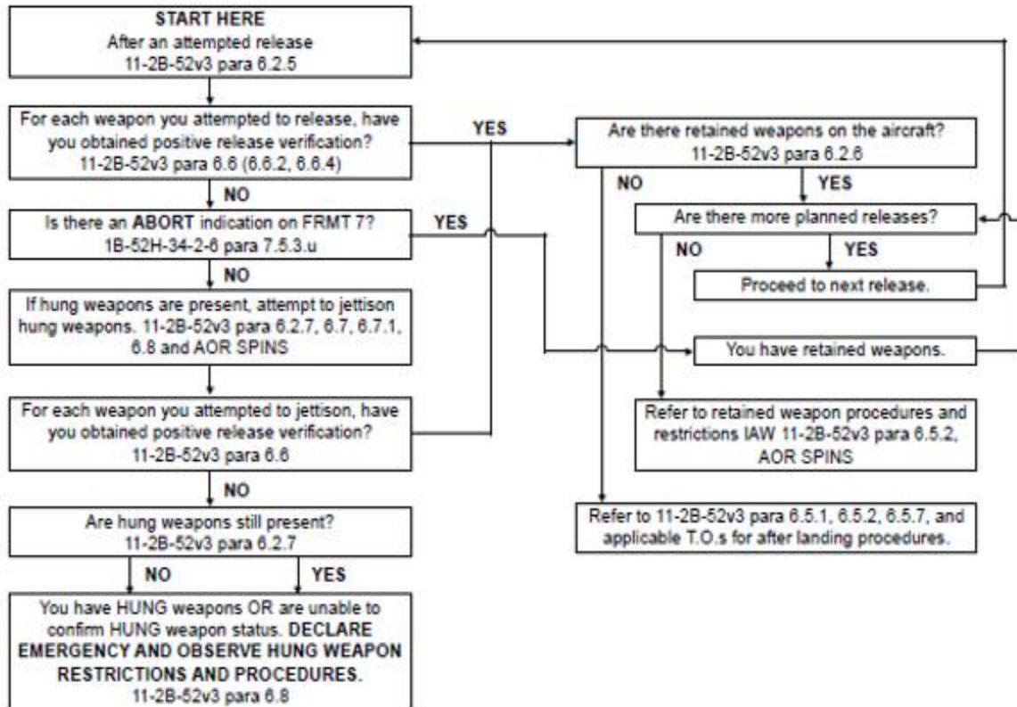
Figure A11.1. (Added-MINOTAFB) Weapons Flow Chart.
