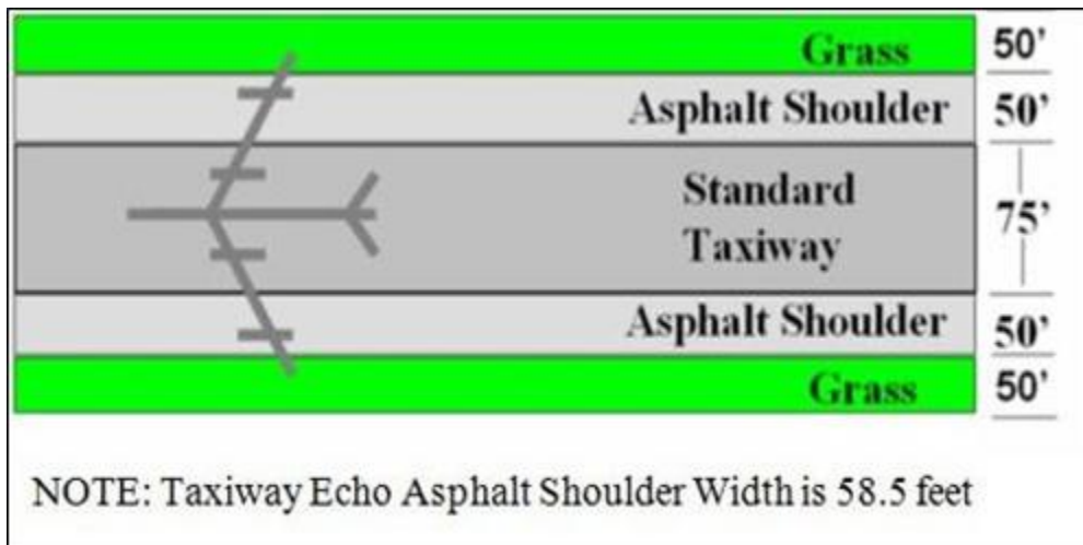
Figure A9.3. (Added-MINOTAFB) Taxiway Wingtip Clearance.
