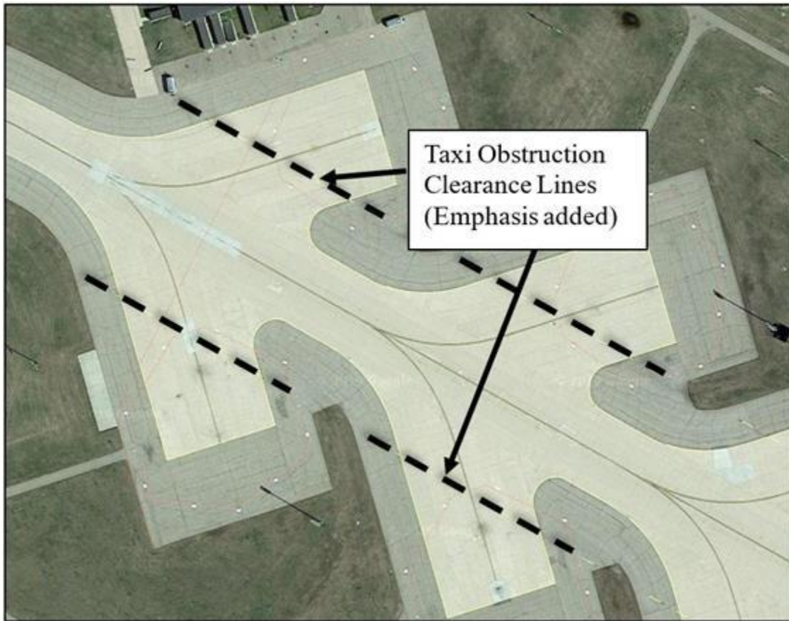
Figure A9.2. (Added-MINOTAFB) APA Taxi Obstruction Lines.
