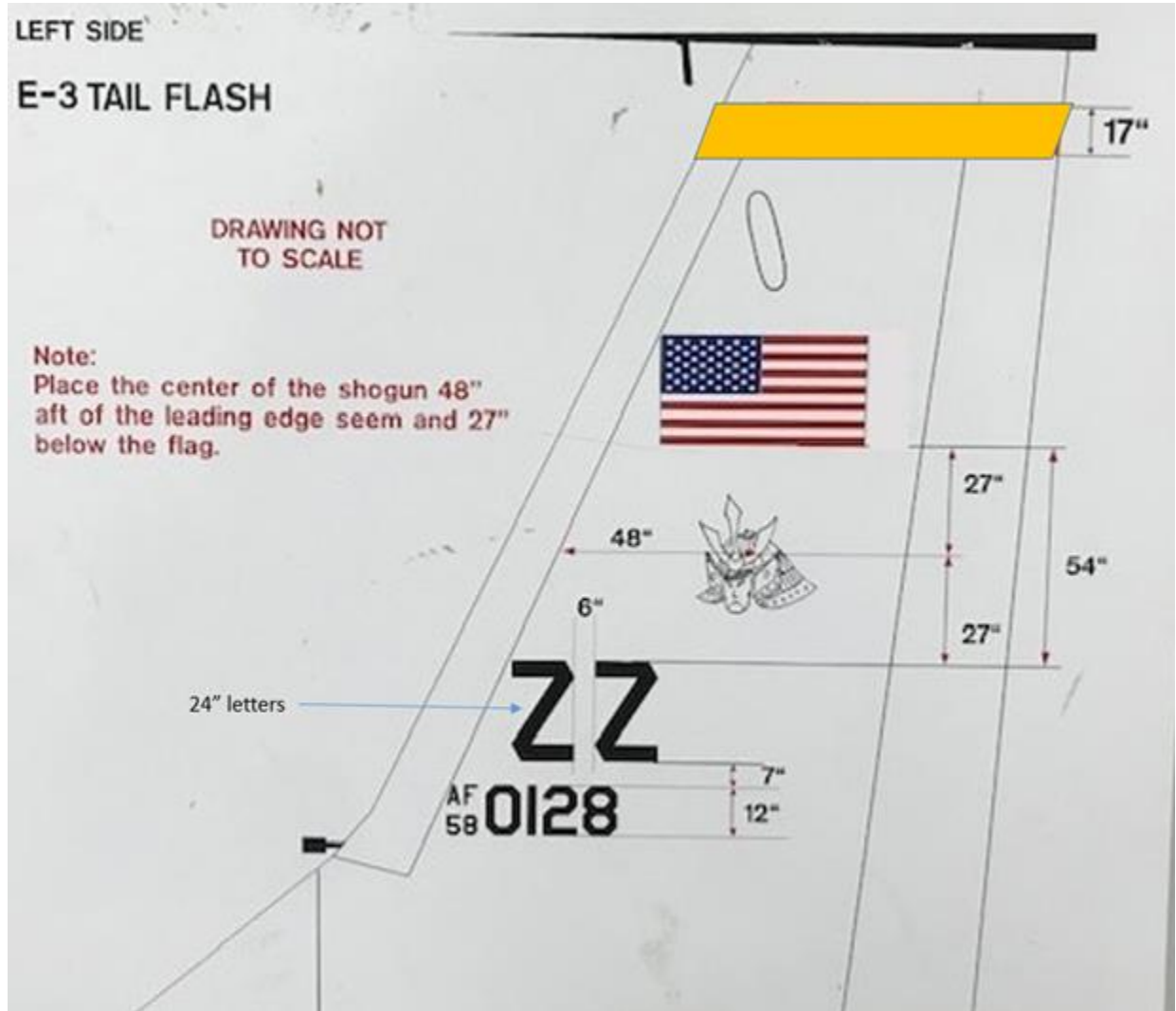
Figure A16.1. (Added-KADENAAB) 961 AACCS Standard E-3 Configuration.
