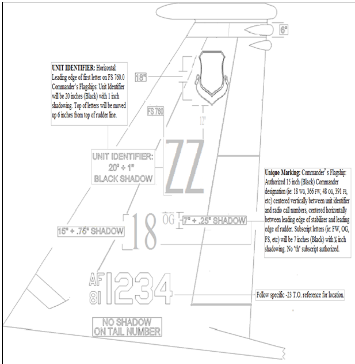
Figure A10.1. (Added-KADENAAB) 18 OG Commander's Tail Configuration.
