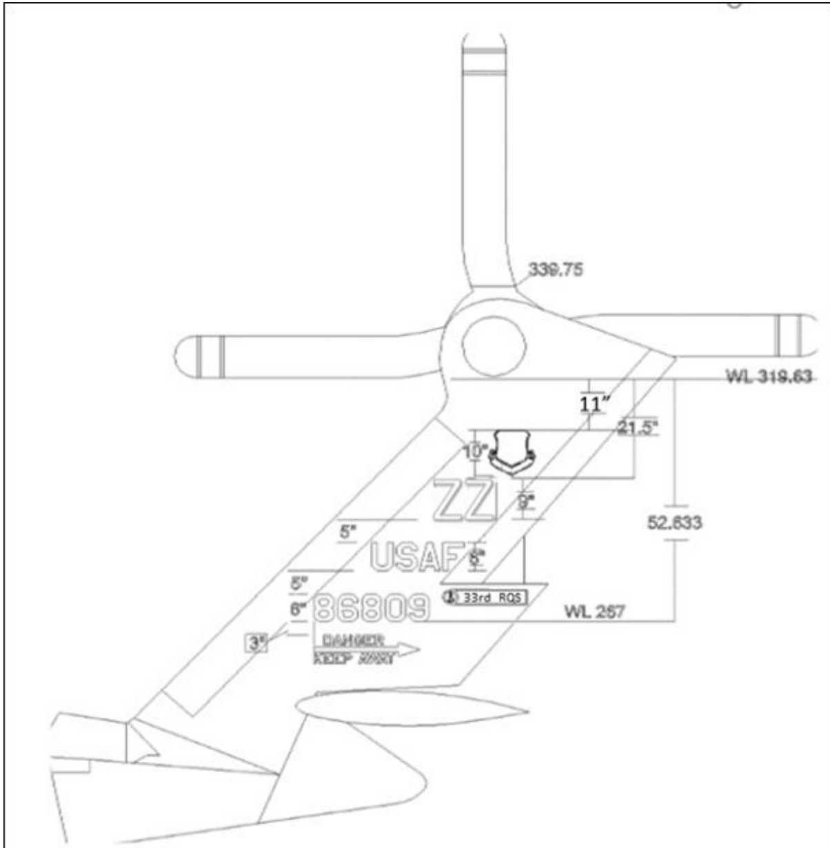
Figure A18.1. (Added-KADENAAB) 33 RQS Tail Configuration for HH-60 Left Tails.
