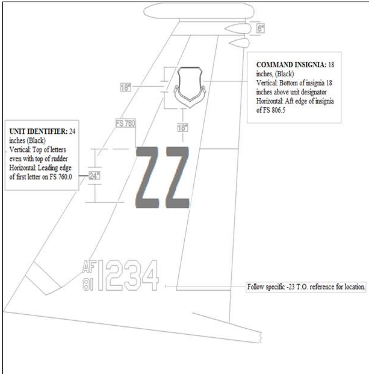
Figure A8.1. (Added-KADENAAB) 67FS Standard F-15 Tail Configuration.
