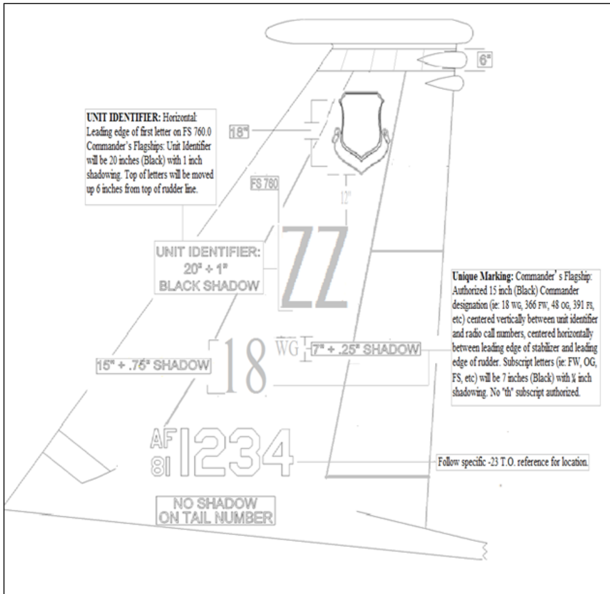
Figure A12.1. (Added-KADENAAB) 18 WG Commander's Tail Configuration.
