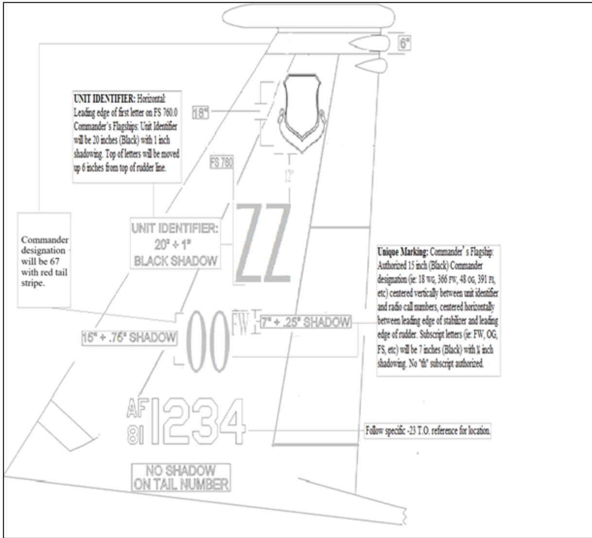
Figure A9.1. (Added-KADENAAB) 67 FS Commanders' Tail Configuration.
