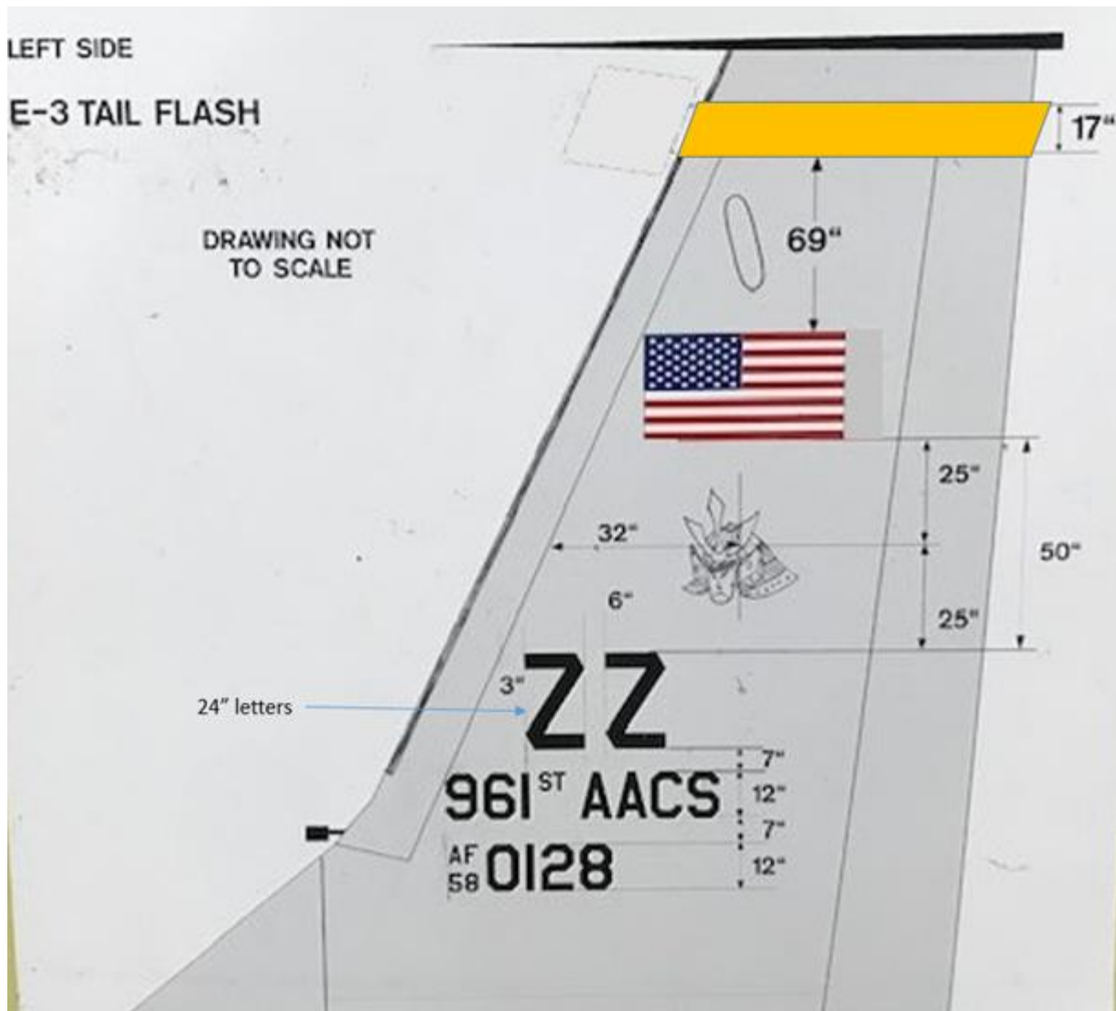
Figure A17.1. (Added-KADENAAB) 961 AACS Commander's E-3 Configuration.
