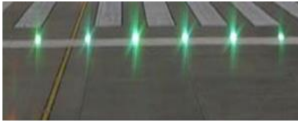
Figure 4.34. (Added-EDWARDSAFB) .Runway Threshold Lights.
