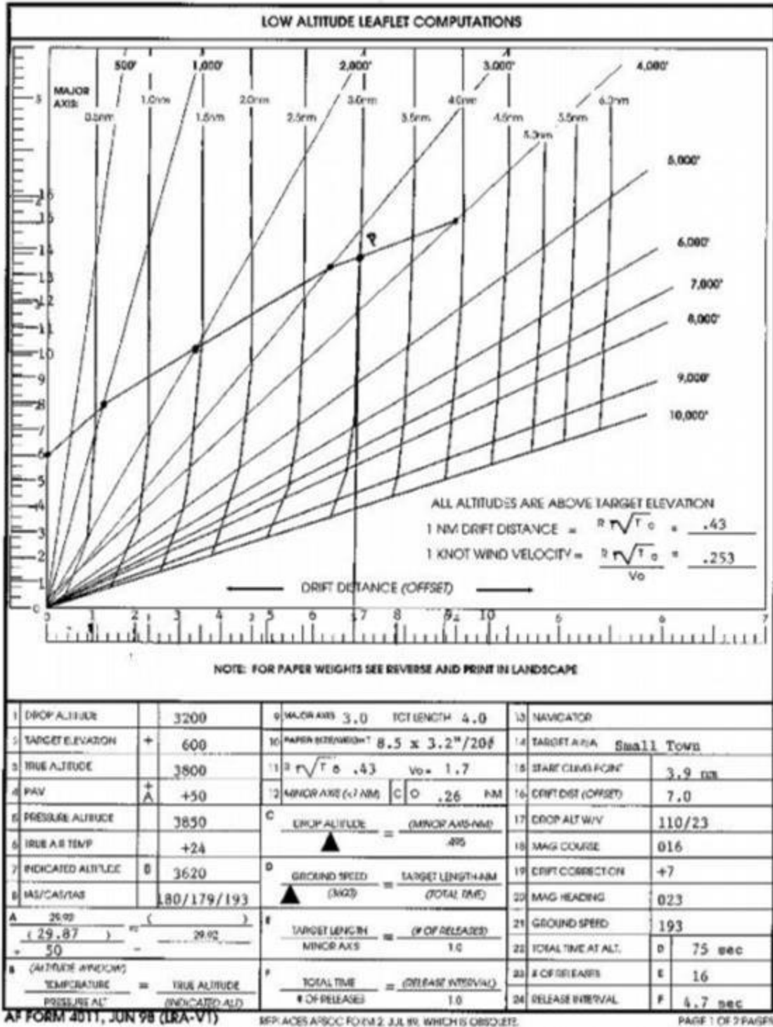
Figure A3.1. (AFSOC) AF Form 4011 Low Altitude Leaflet Computation.
