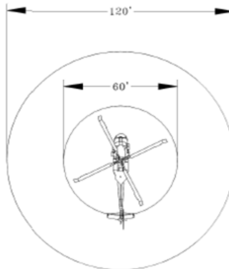
Figure A6.4. HH-60 Helicopter Landing Zone Size.
