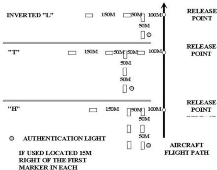
Figure 2.6. Ground Marked Release System Day and Night Markings.
