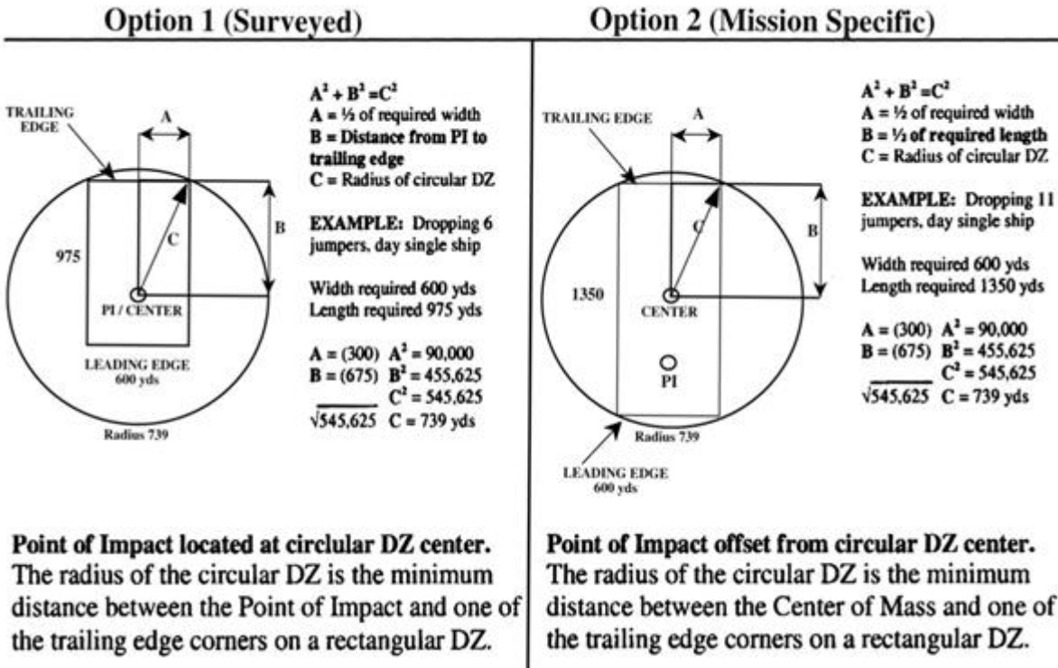
Figure 2.1. Circular Drop Zone Computation. (The new figure correctly shows the length of both line segment Bs to the trailing edge of the DZ.)
