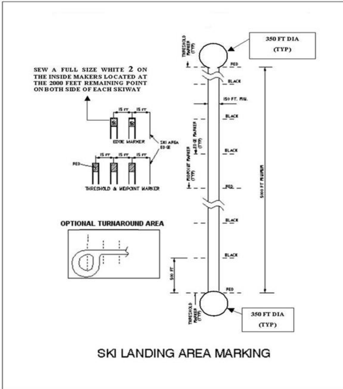
Figure 4.4. Ski Landing Area Marking.
