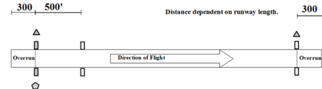
Figure 3.5. Airfield Marking Pattern - 3 (Day).
