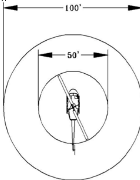
Figure A6.3. UH-1 Helicopter Landing Zone Size.
