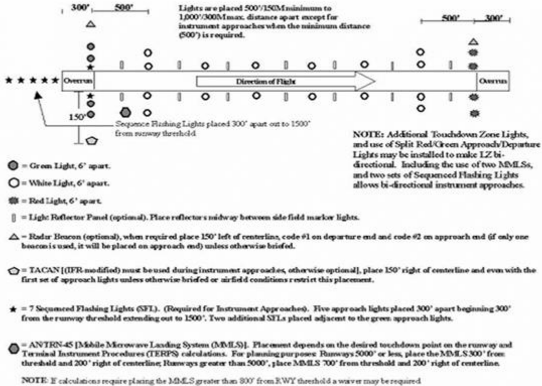
Figure 3.3. Airfield Marking Pattern - 2 (Day).
