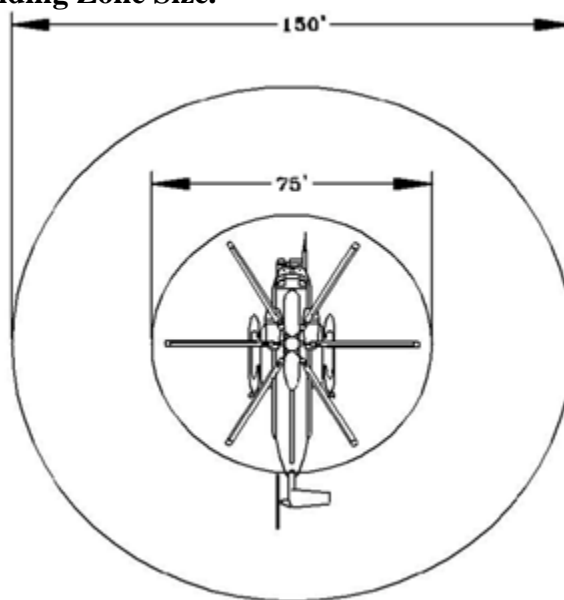
Figure A6.1. MH-53 Helicopter Landing Zone Size.
