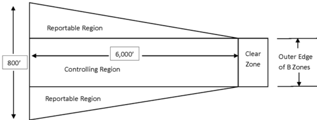
Figure 3.9. (Added-AFSOC) . LTFW Aircraft Approach Zone.
