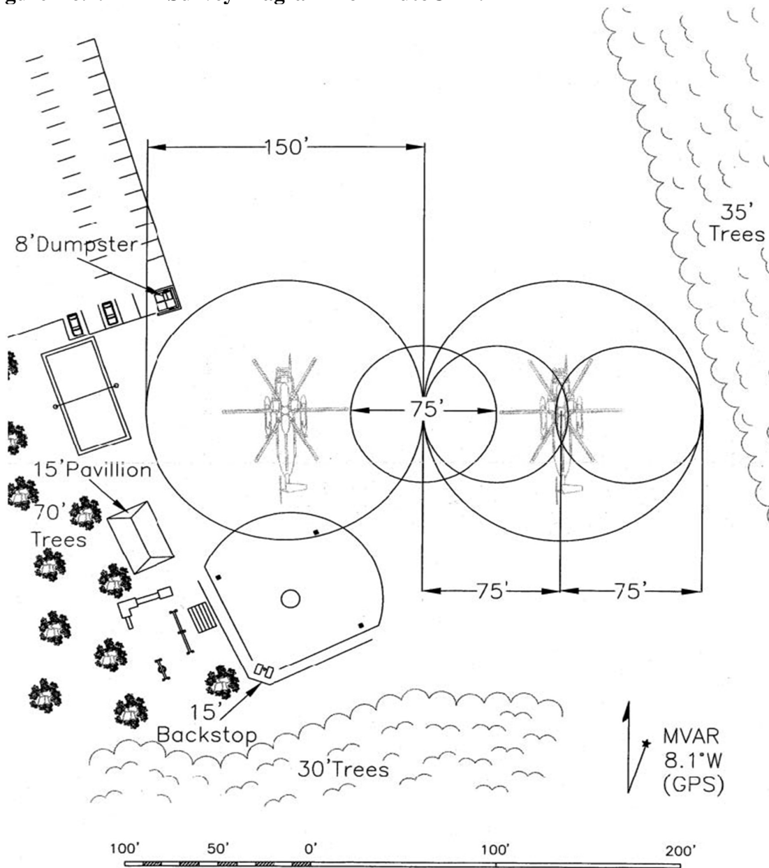
Figure A6.7. HLZ Survey Diagram from AutoCAD.
