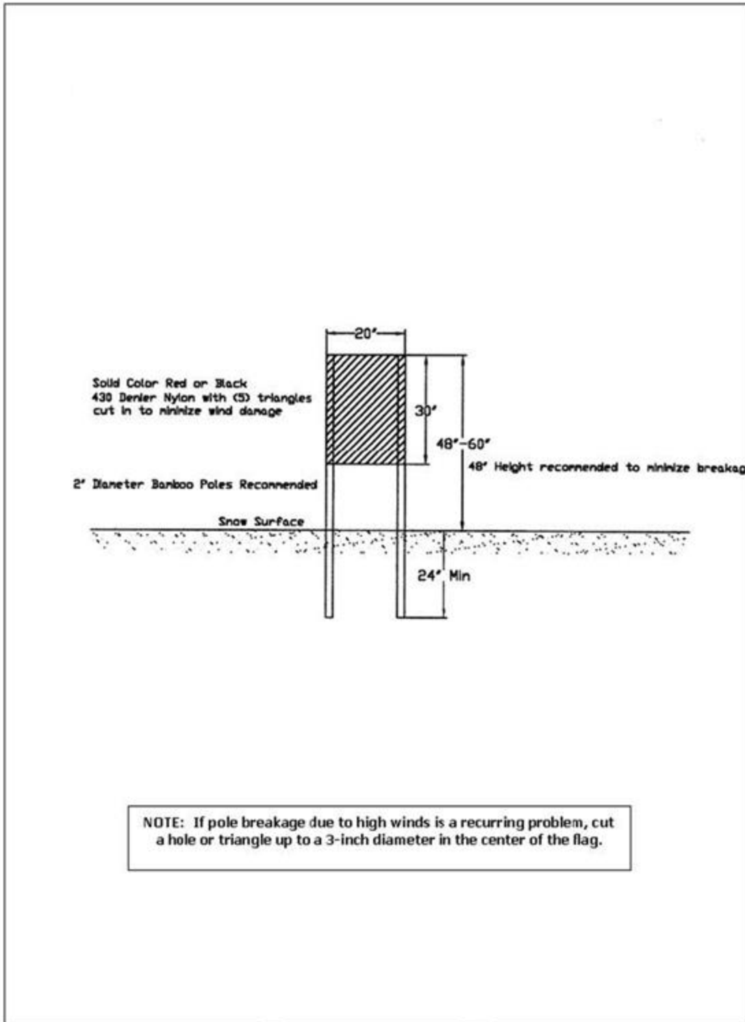
Figure 4.3. Typical Skiway Marker Construction.
