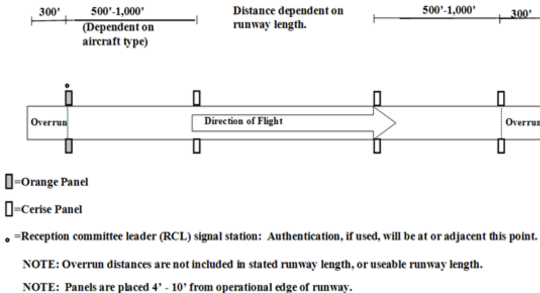
Figure 3.3. Airfield Marking Pattern - 2 (Day).
