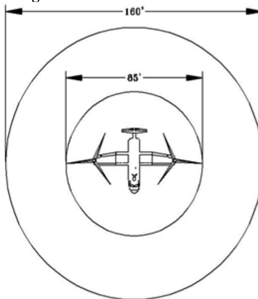
Figure A6.2. CV-22 Helicopter Landing Zone Size.
