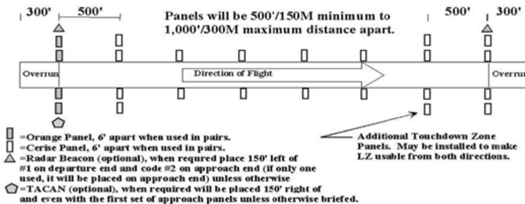
Figure 3.1. Airfield Marking Pattern - 1 (Day).
