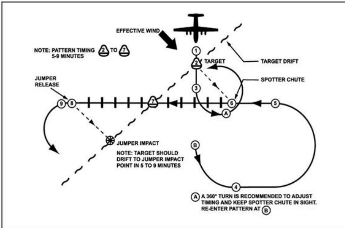
Figure 2.5. Jumpmaster Directed Airdrop, Moving Target Procedures.
