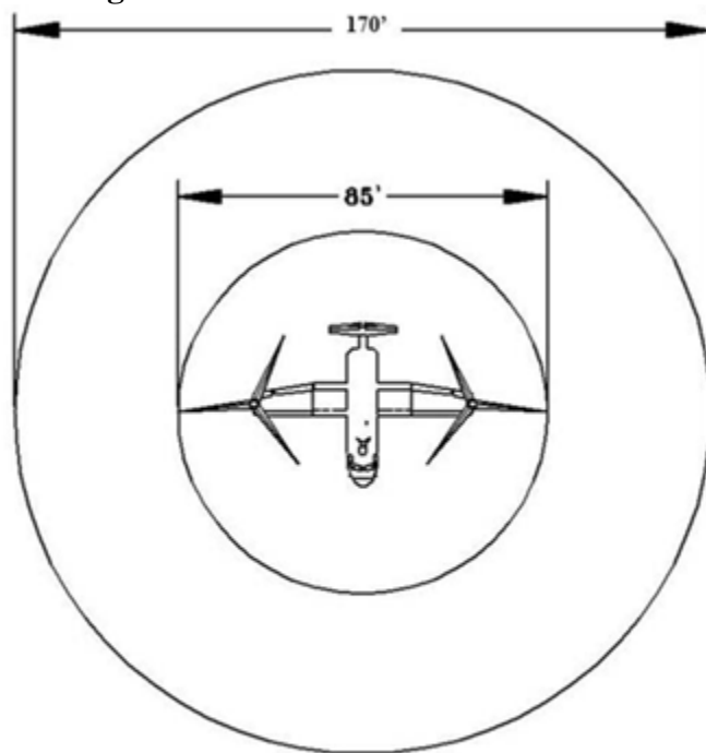
Figure A6.2. (AFSOC) CV-22 Helicopter Landing Zone Size.
