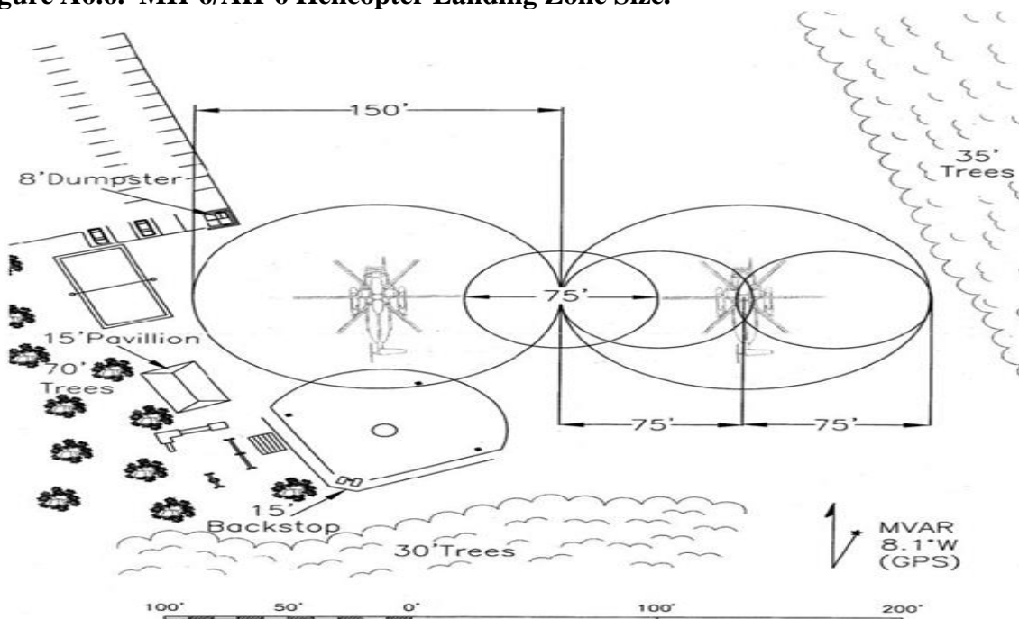
Figure A6.6. MH-6/AH-6 Helicopter Landing Zone Size.
