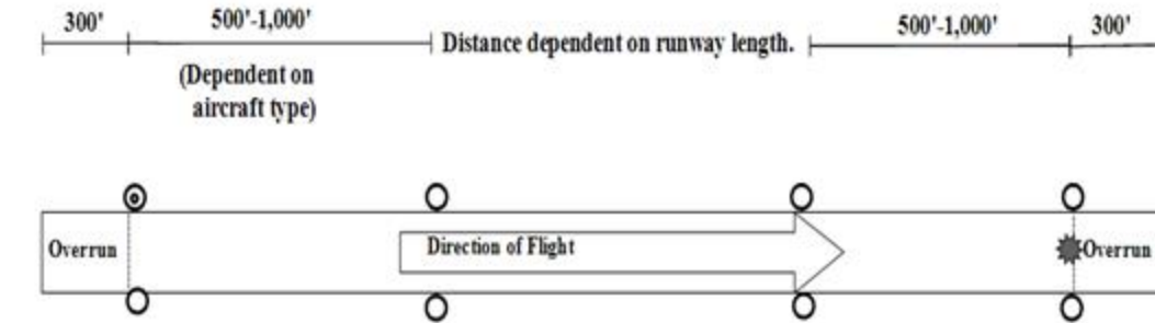
Figure 3.4. Airfield Marking Pattern - 2 (Night).
