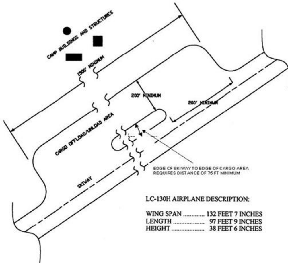
Figure 4.2. Cargo Offload/Onload Area.
