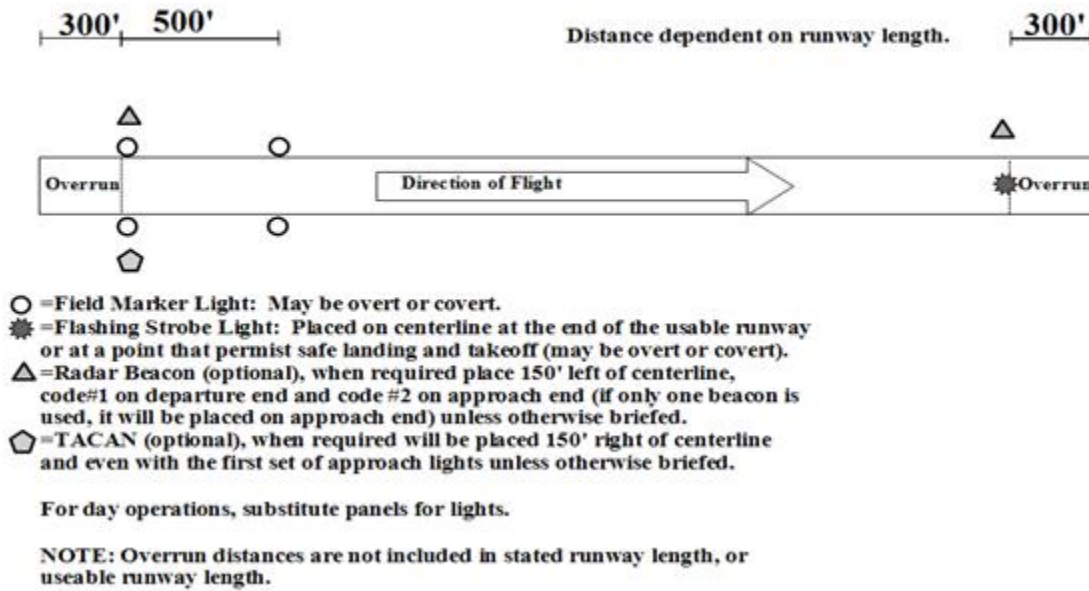
Figure 3.6. (AFSOC) Airfield Marking Pattern - 3 (Night).
