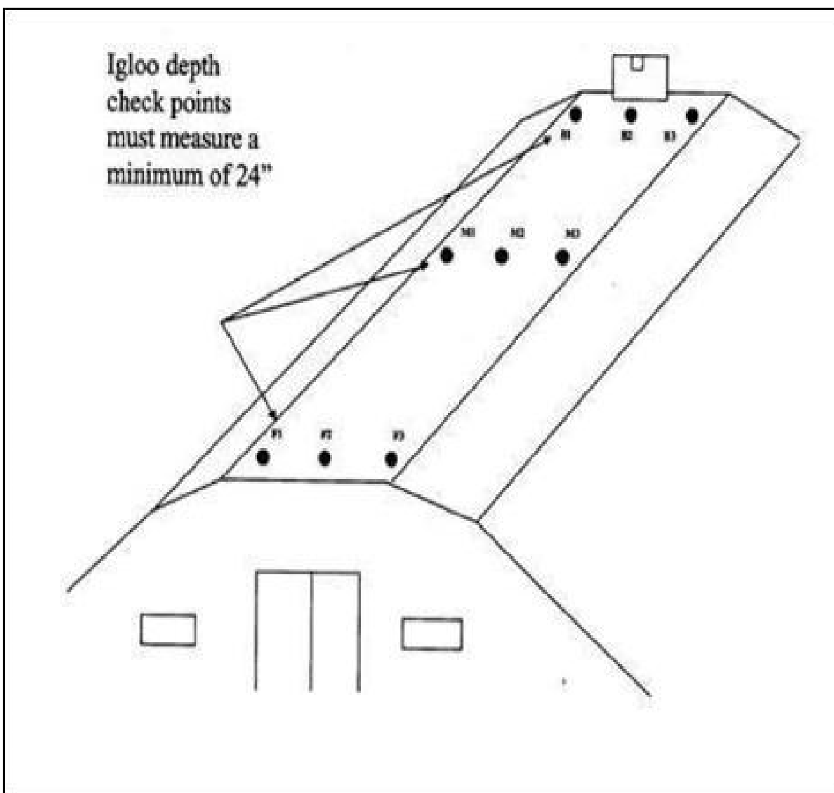
Figure V2.E5.F7. (Added-AFMC) SAMPLE – Annual Earth Covered Igloo Depth Check Diagram
