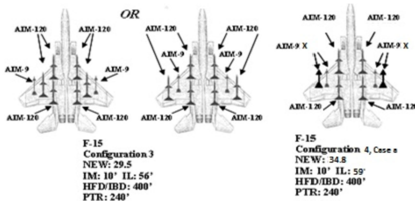
Figure V4.E3.F2. (Added)(DAF) Reduced MCEs and QDs for F-15 Aircraft in the Open.
