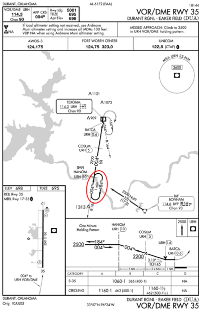
Figure 15.26. HILPT Approach.
