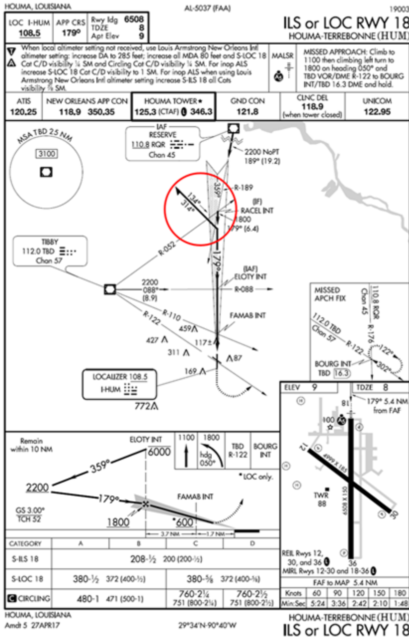
Figure 15.17. Procedure Turn.
