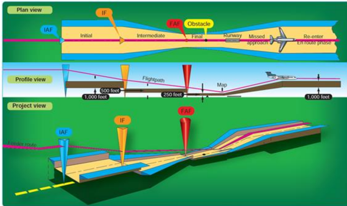
Figure 15.10. Approach Segments.
