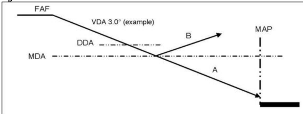
Figure 16.5. CDFA.
