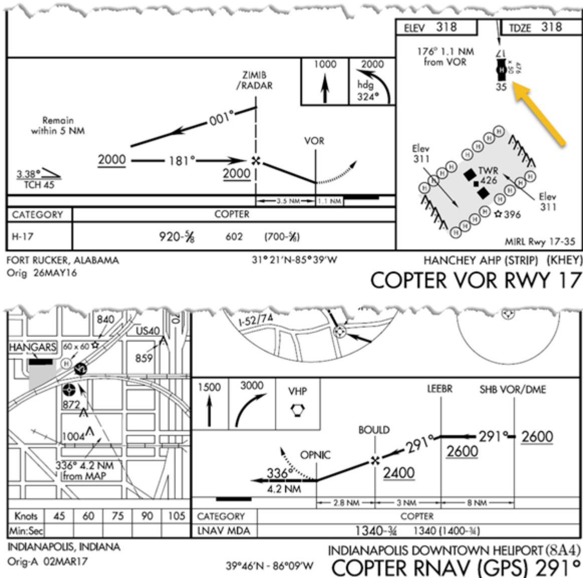
Figure 15.30. Helicopter-Only Approach.
