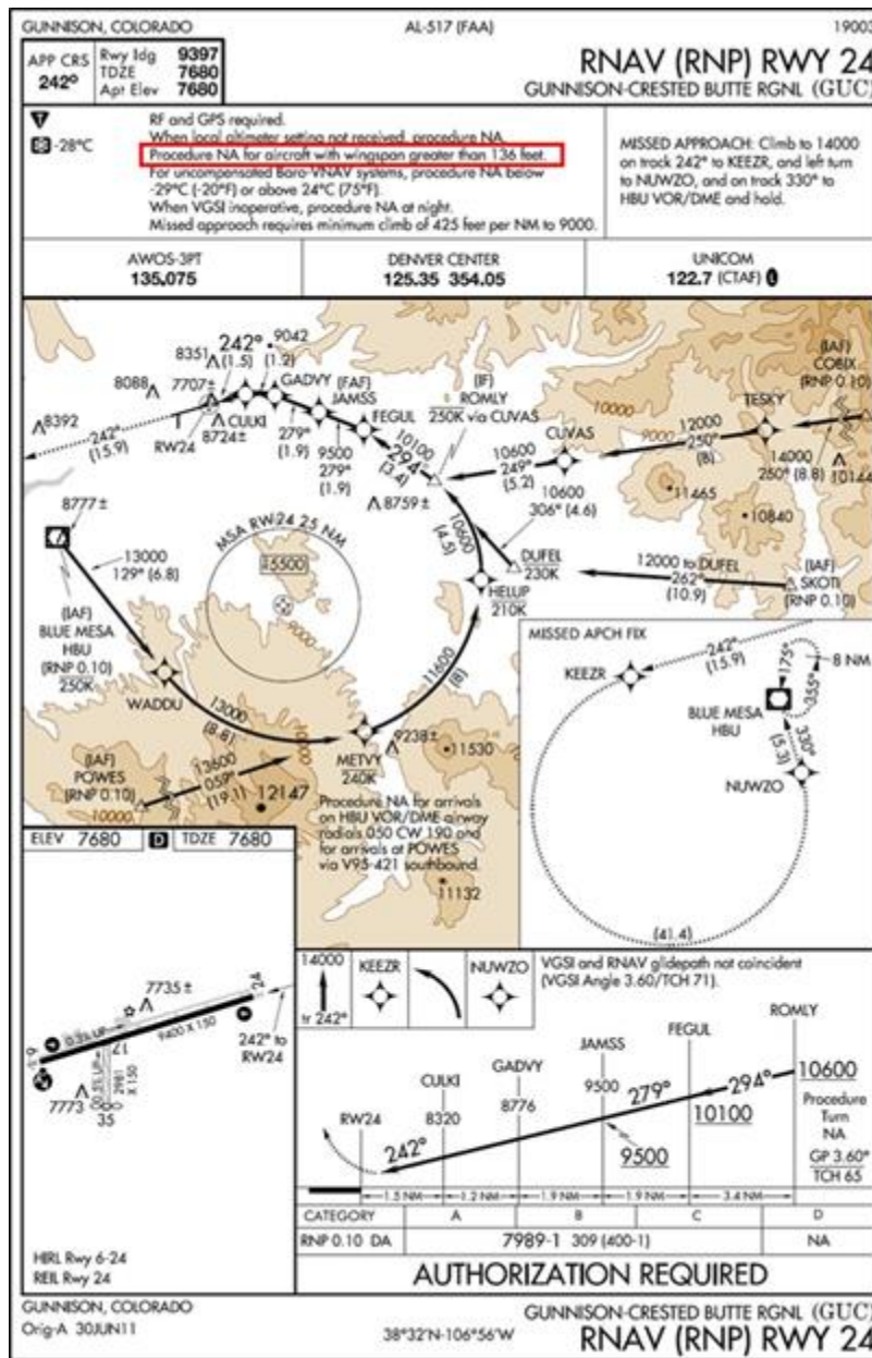
Figure 17.8. Aircraft Size Restrictions.
