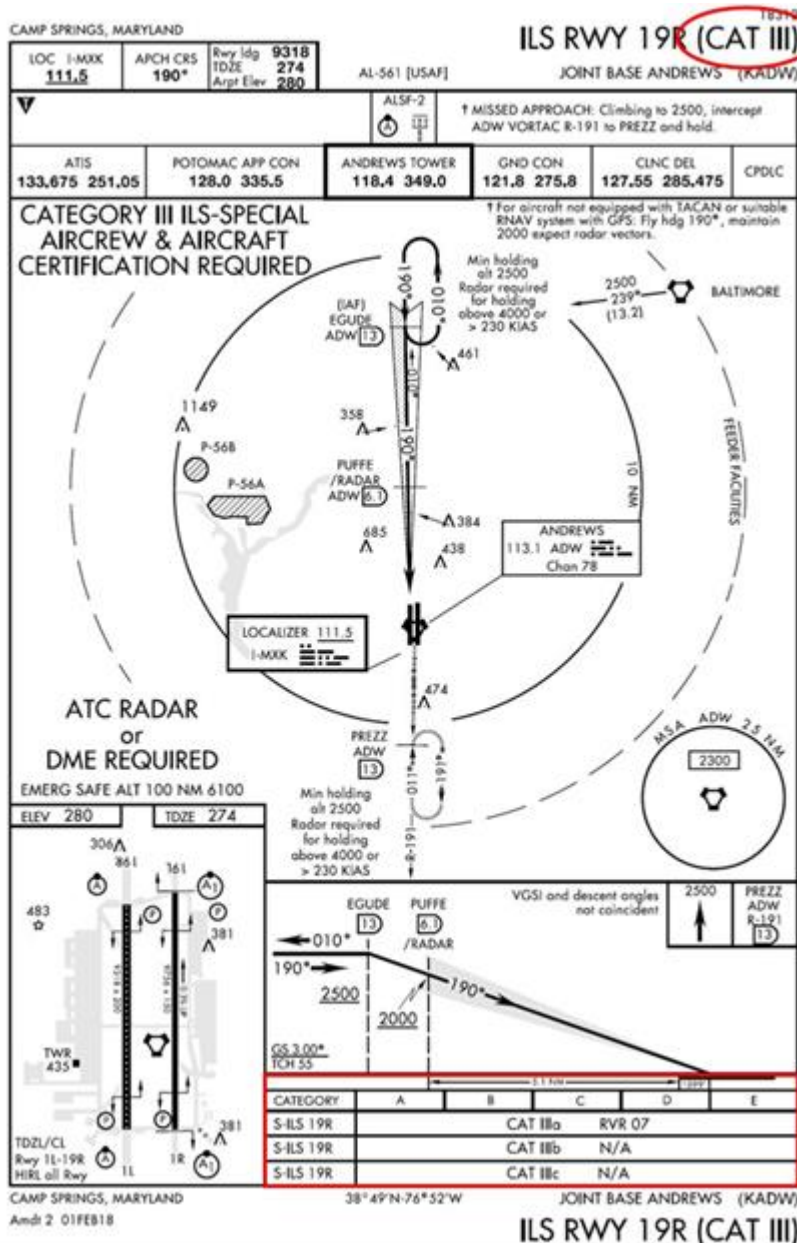
Figure 17.5. CAT III ILS Approach.
