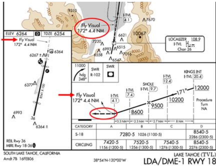
Figure 16.10. Visual Segment.
