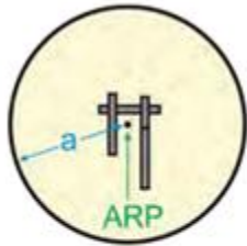
Figure 5.12. Visual Climb Area.
