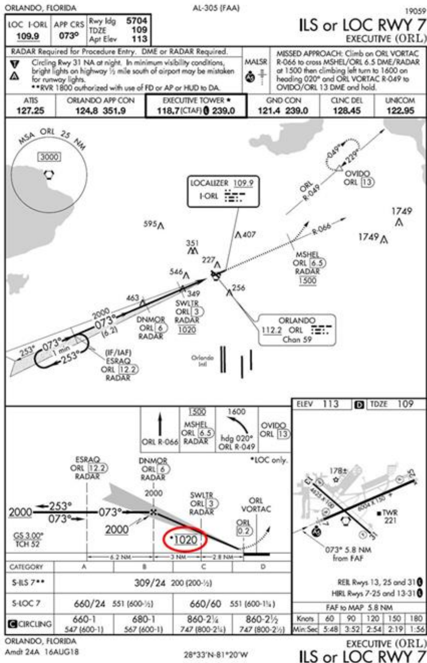
Figure 19.1. Early Missed Approach Restriction.
