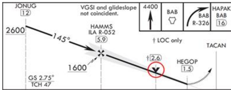
Figure 16.1. VDP.
