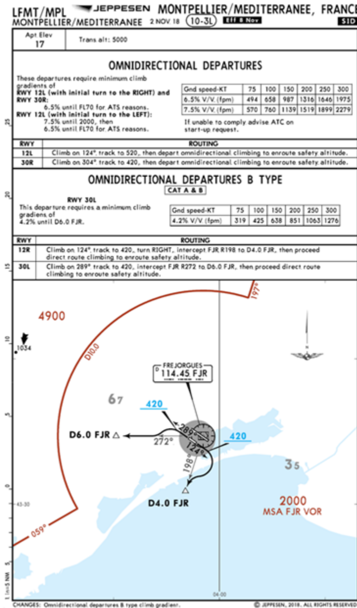
Figure 5.6. Omnidirectional Departure.
