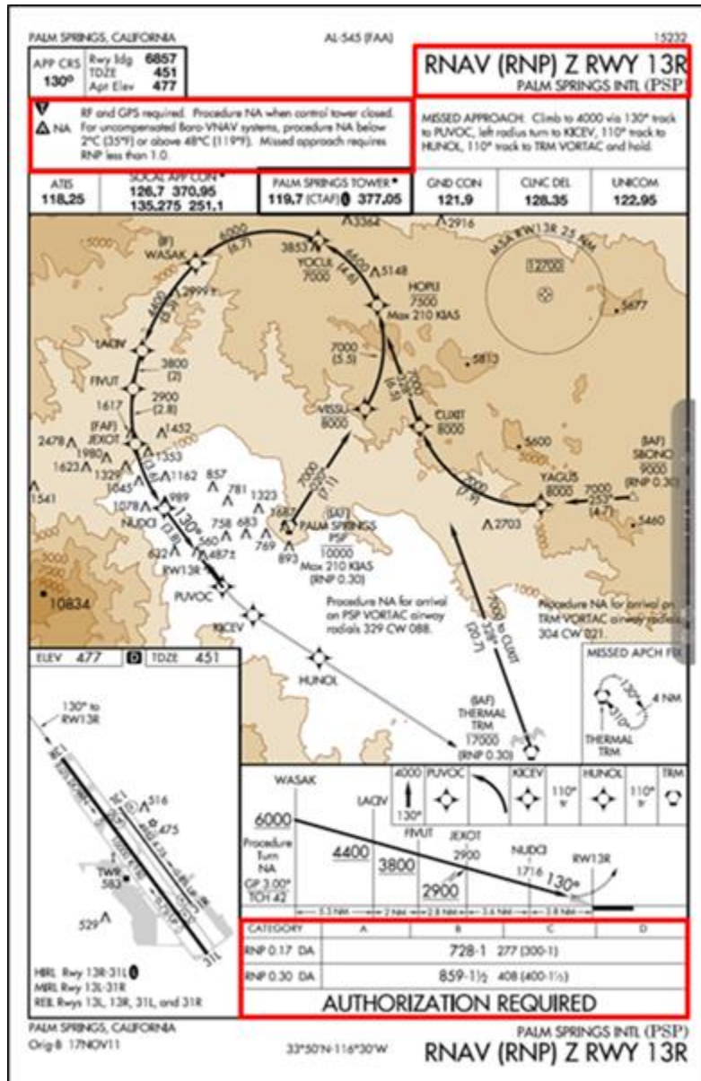
Figure 17.6. RNP Values.
