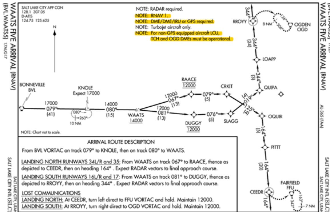
Figure 14.1. RNAV Arrival.
