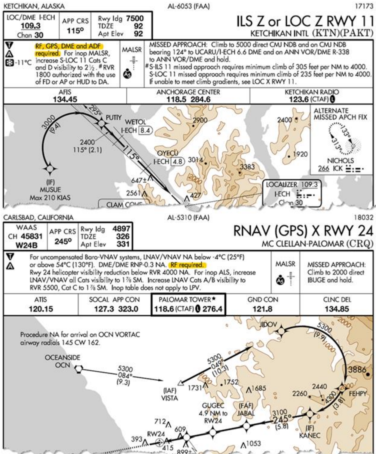
Figure 10.4. Radius-to-Fix (RF) Legs.
