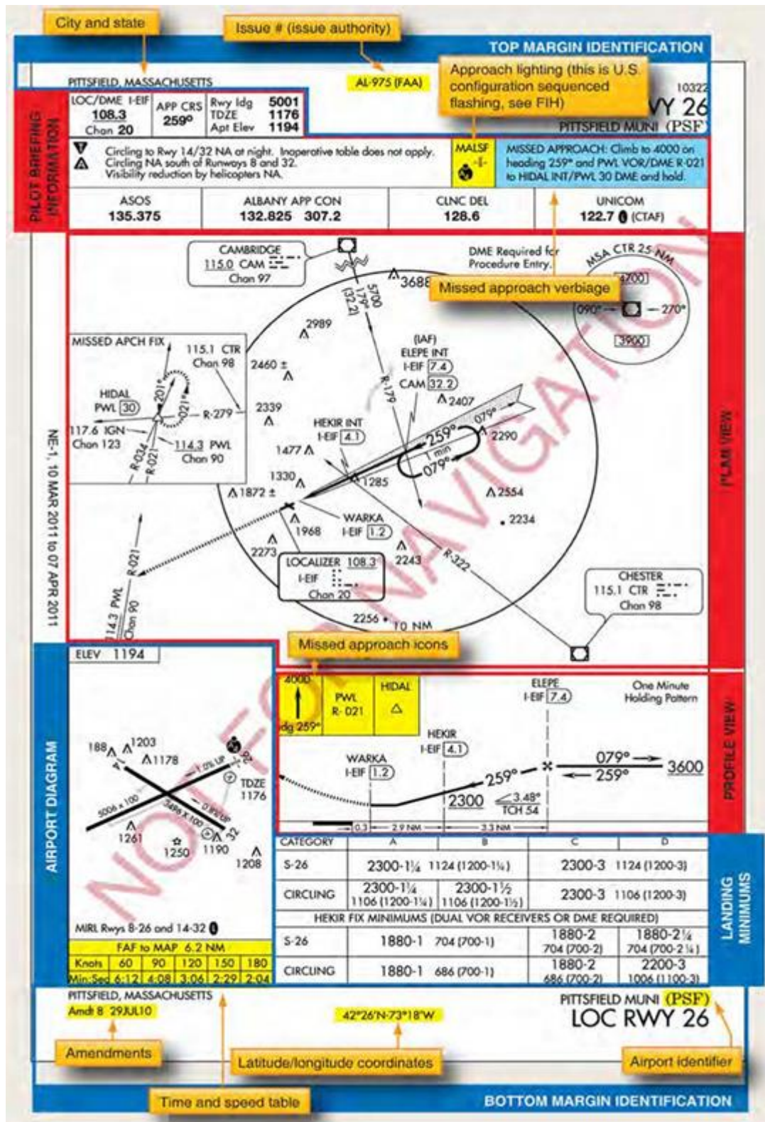
Figure 15.4. Instrument Approach Chart.
