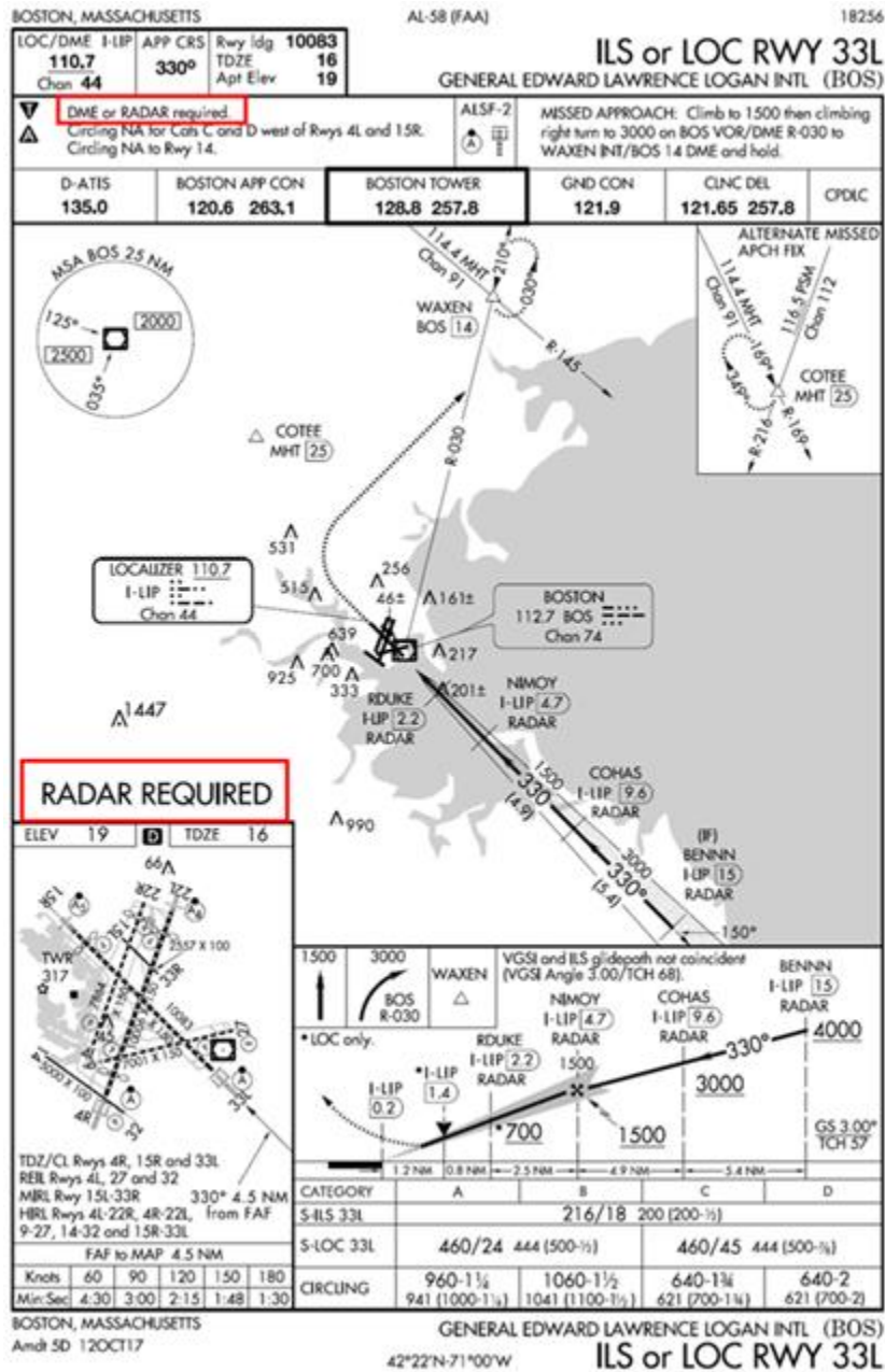
Figure 15.2. Additional Equipment Required for Approach.
