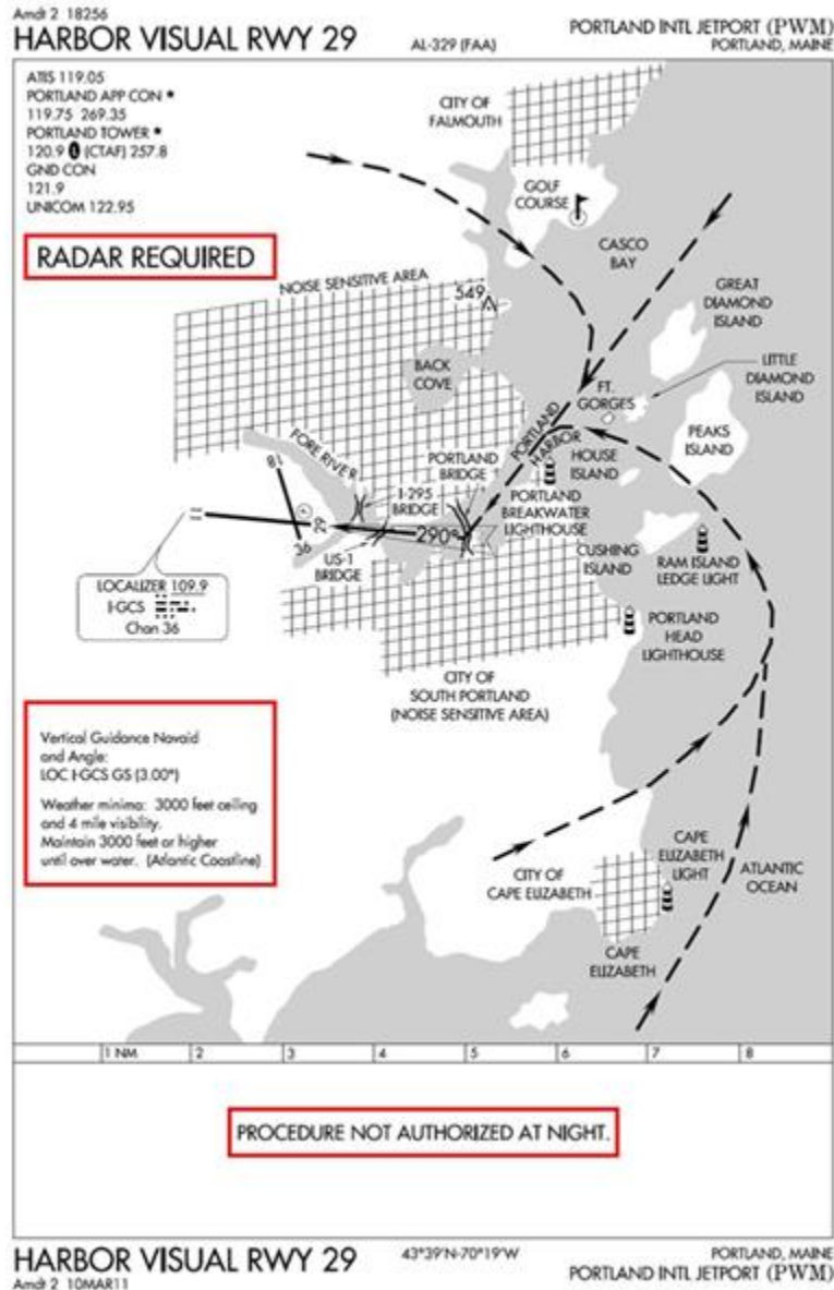
Figure 15.34. Charted Visual Flight Procedure.
