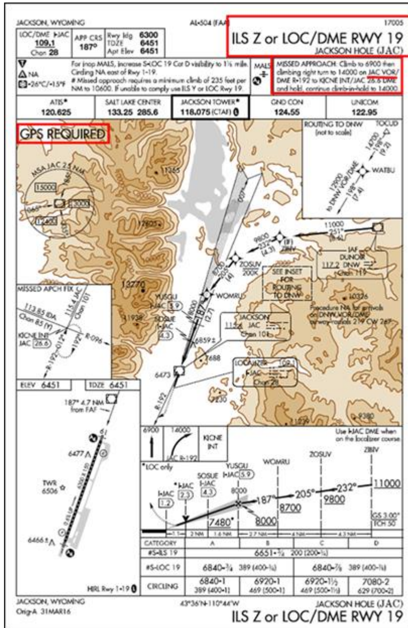
Figure 15.1. Equipment Required for an Approach.
