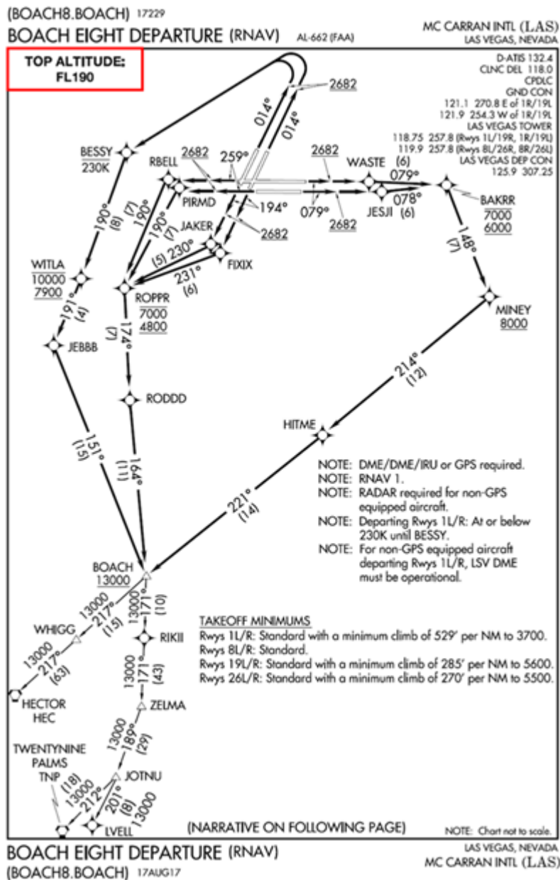
Figure 5.19. Civil SID with Top Altitude.
