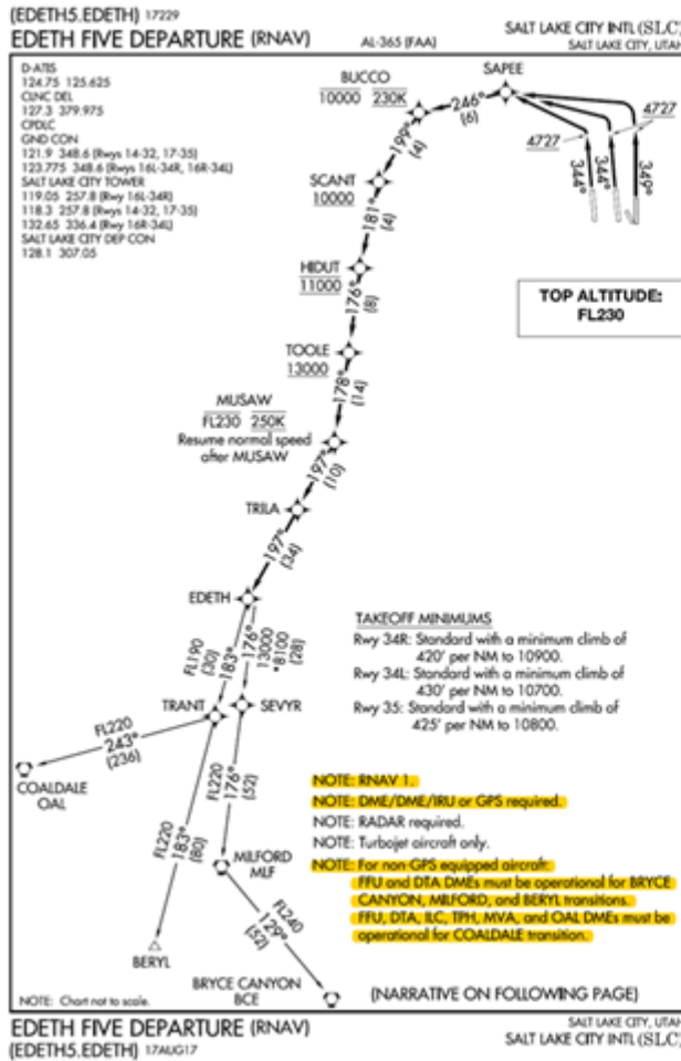
Figure 5.25. RNAV Departure Procedures.
