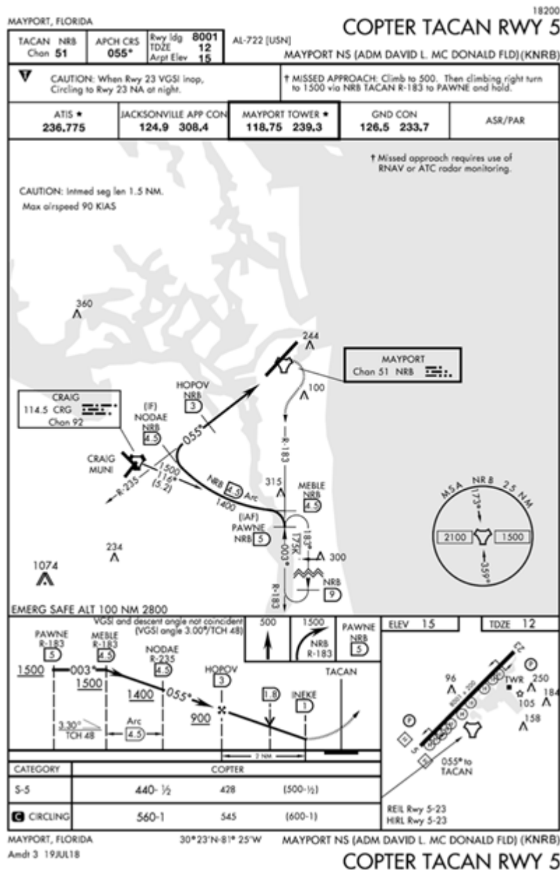
Figure 15.31. Short Final Approach.
