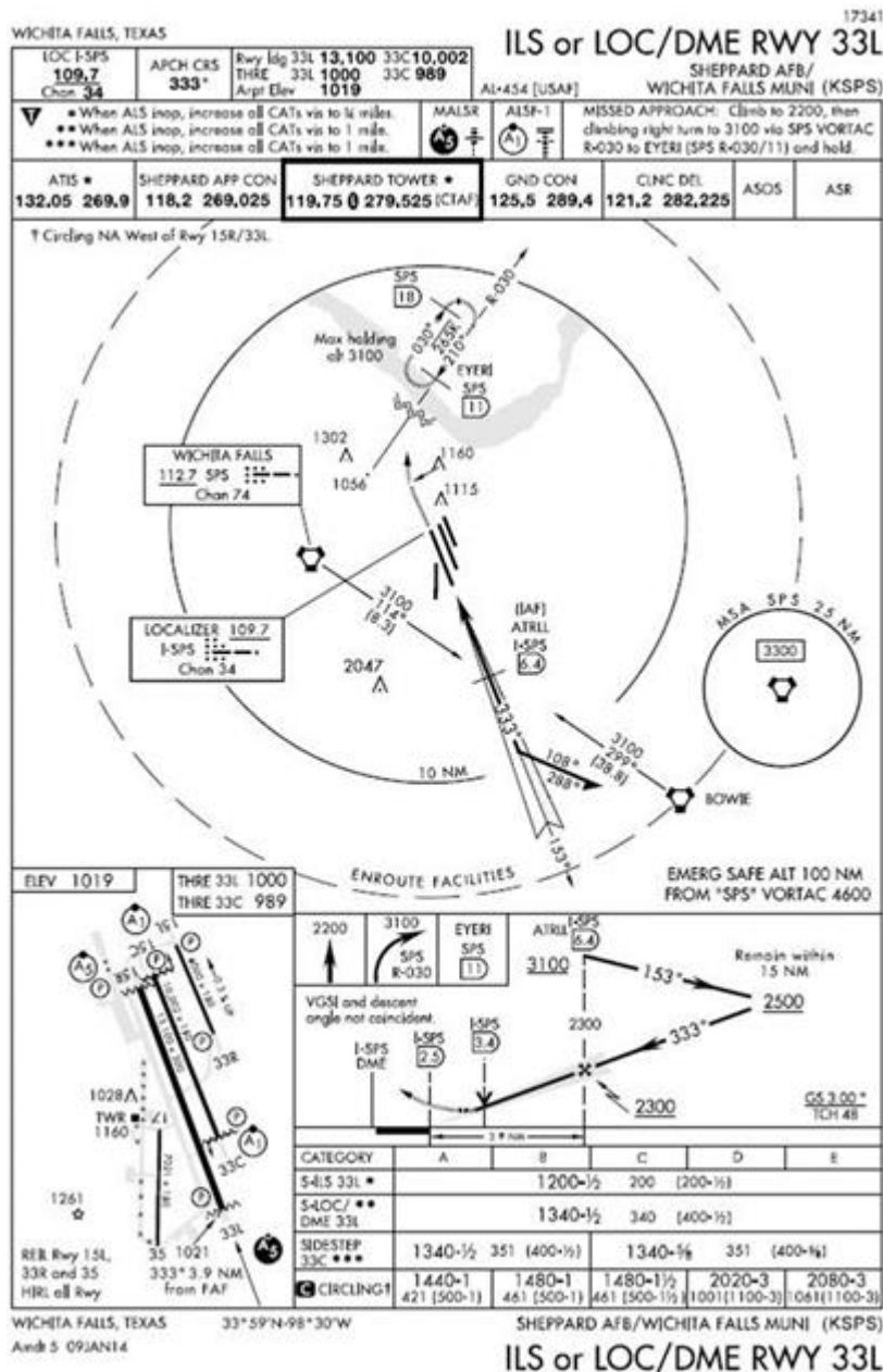
Figure 15.20. Procedure Turn Fix Altitude.
