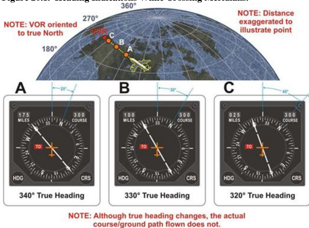
Figure 20.1. Heading Indications While Crossing Meridians.
