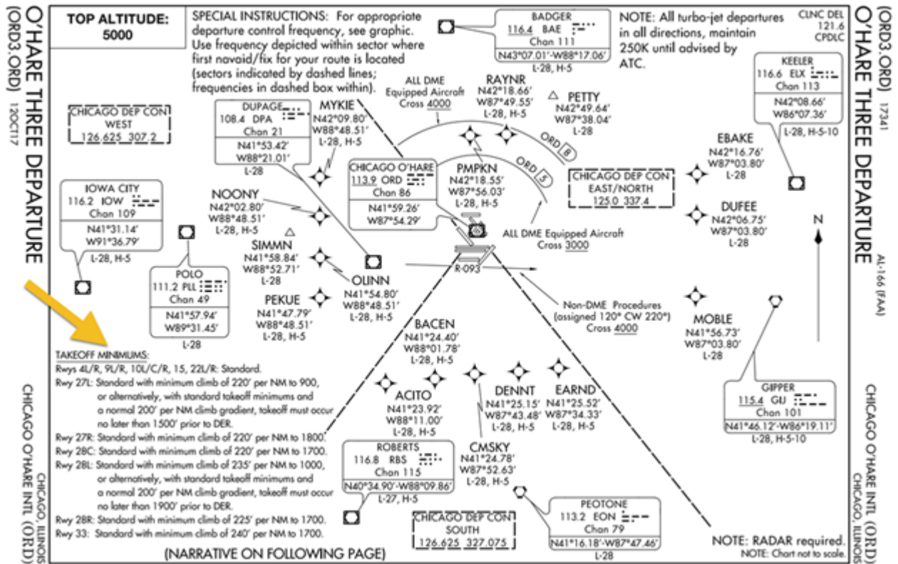
Figure 5.21. Civil SID.
