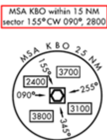
Figure 15.5. Minimum Sector Altitude with Sub-sector Based on Distance.
