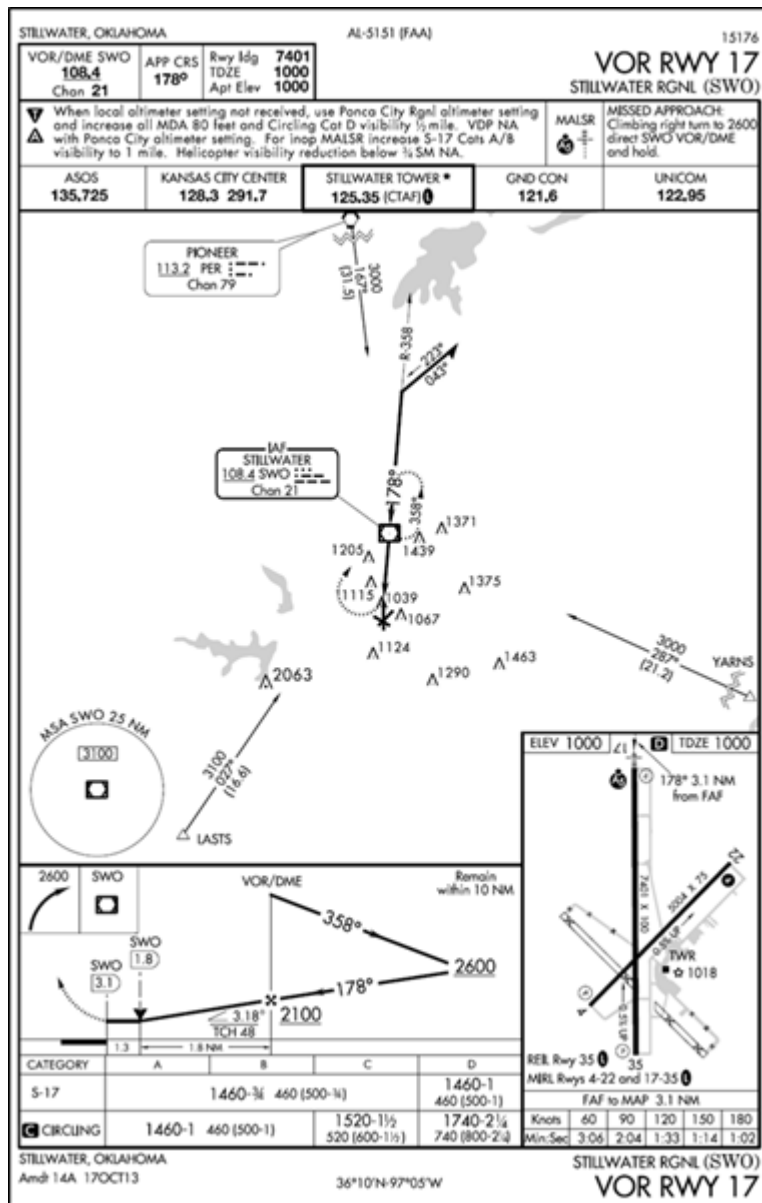
Figure 15.11. Instrument Procedure without a Charted IF.
