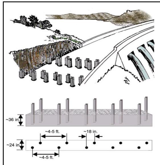
Figure 4.23. Removable Posts.
