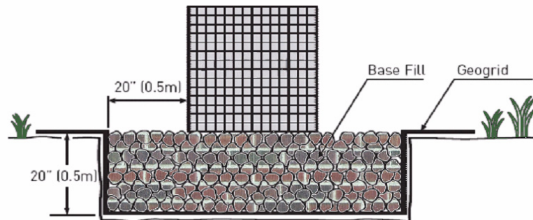
Figure 2.24. Improved Foundation.
