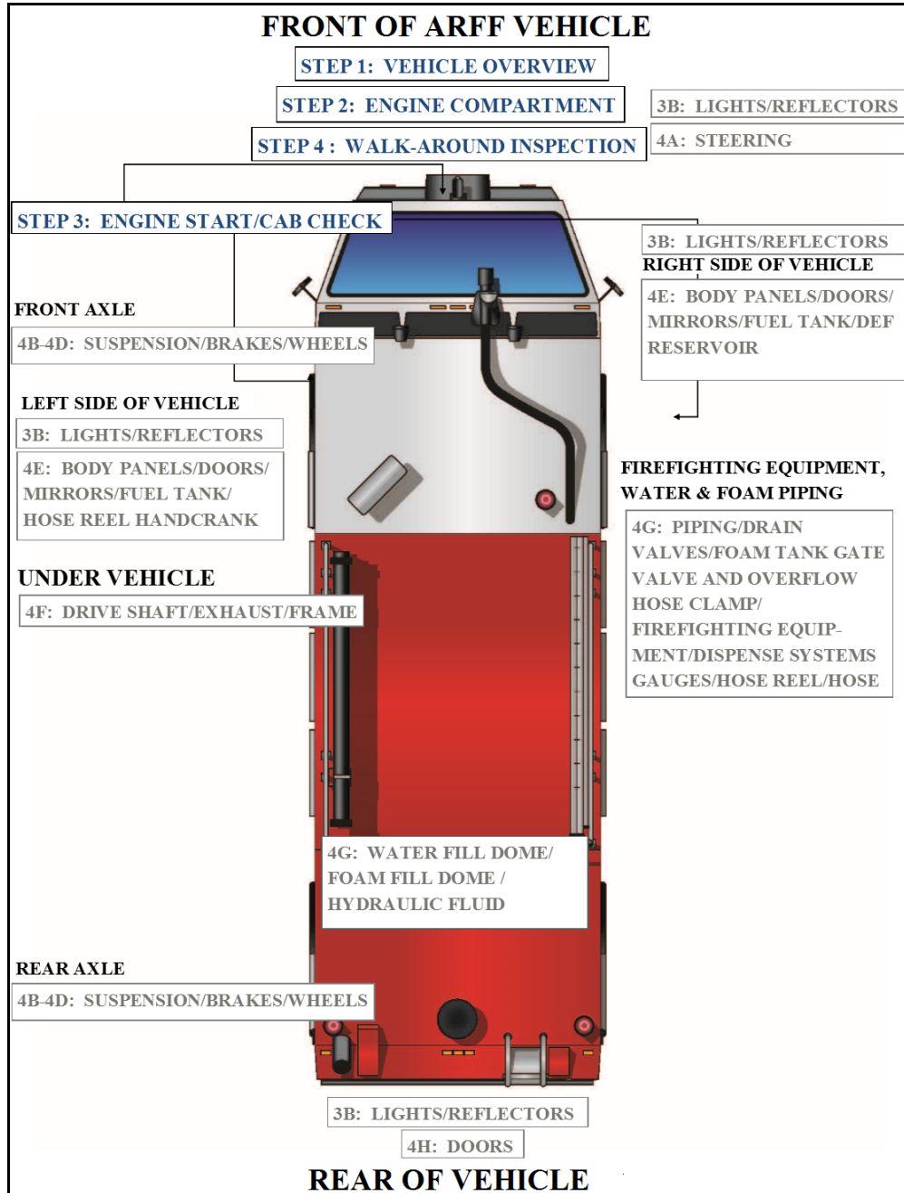
Figure A2.1. Vehicle Inspection Guide.
