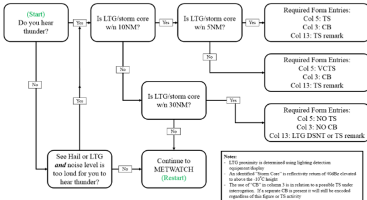
Figure 10.1. Thunderstorm Determination.
