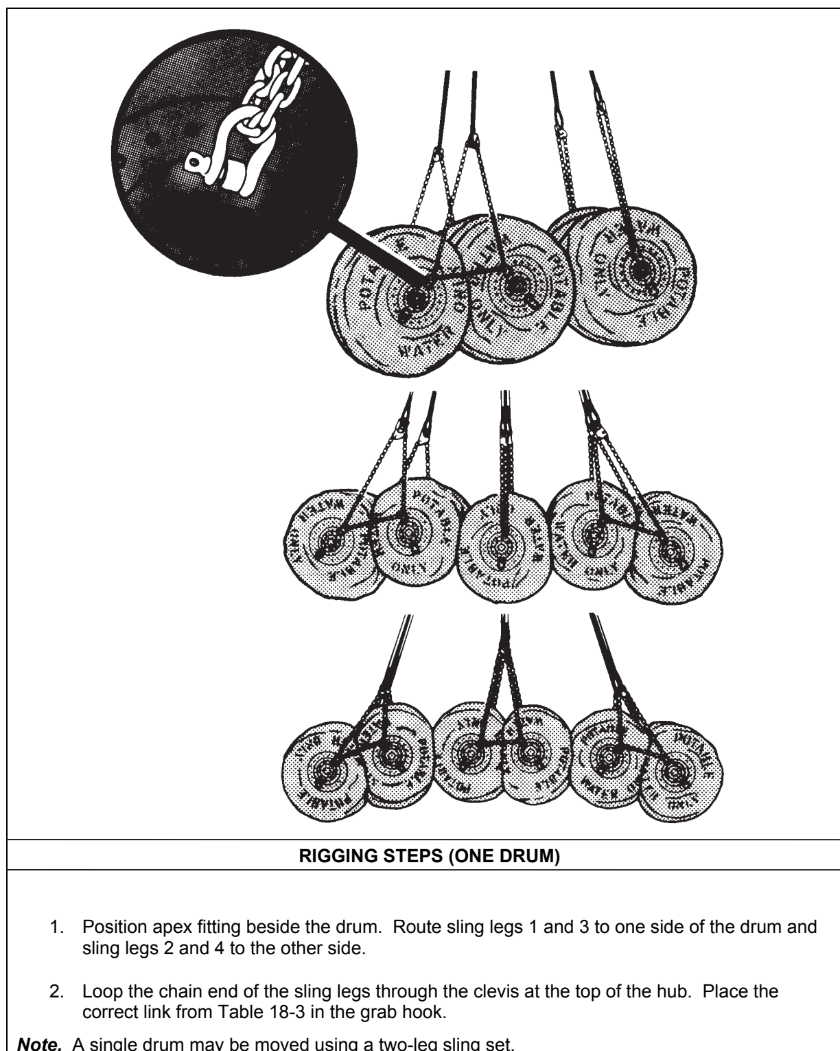
Figure 18-3. One to Six 250-Gallon Water Drums
