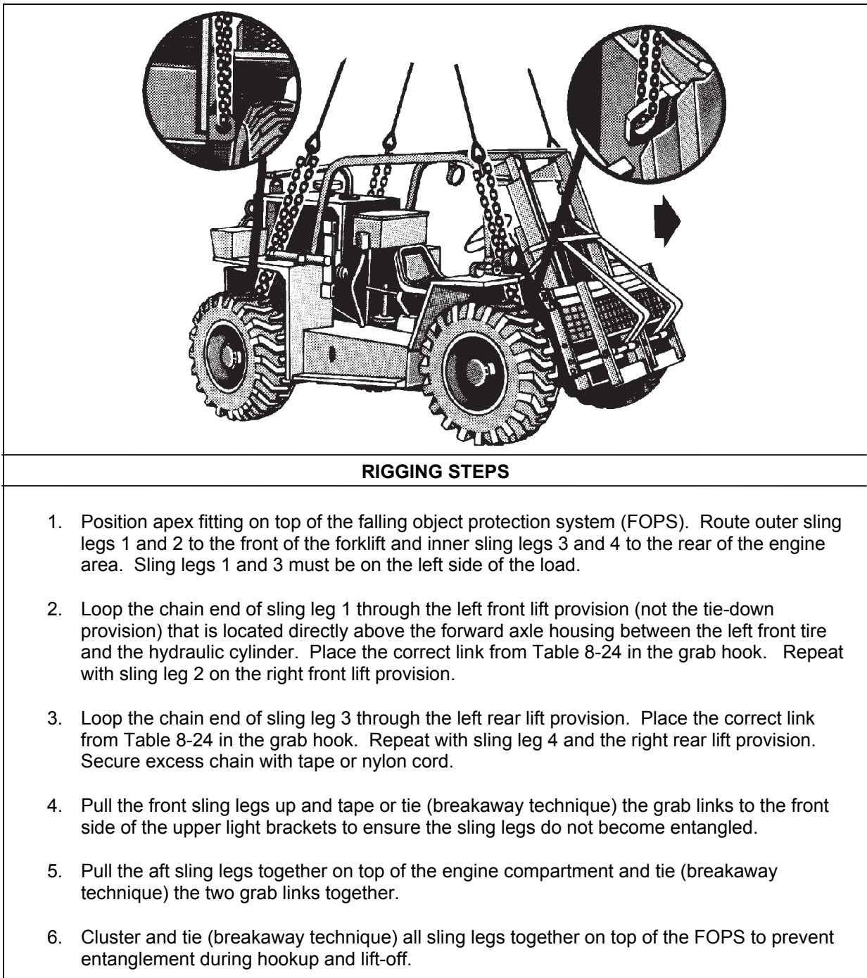
Figure 8-24. Truck, Forklift, MC-4000
