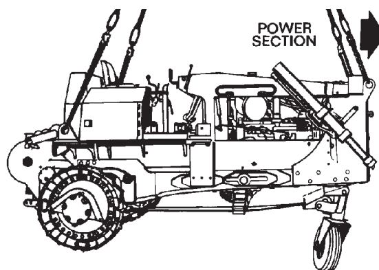
Figure 8-2. D5B Tractor, Dozer, Track Section (Continued)
