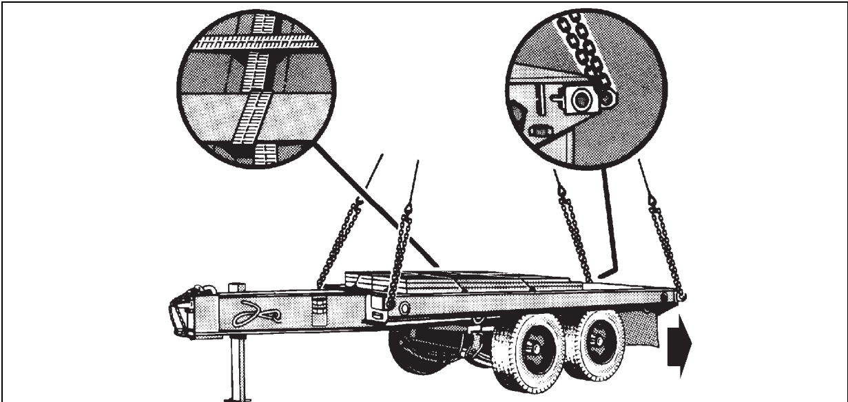
Figure 3-6. M989 HEMAT
