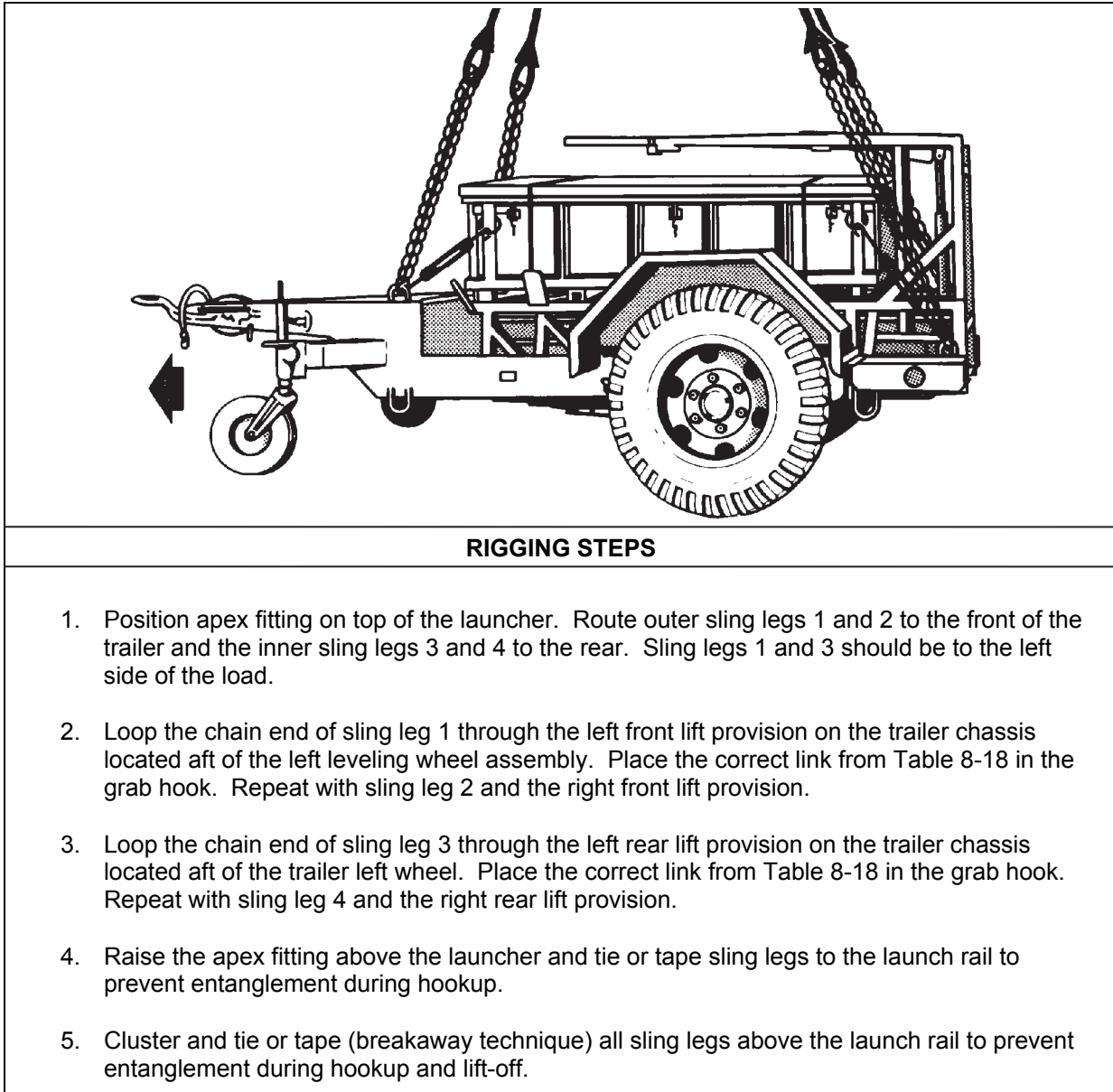
Figure 8-18. Mk155 Launcher on M353 Trailer
