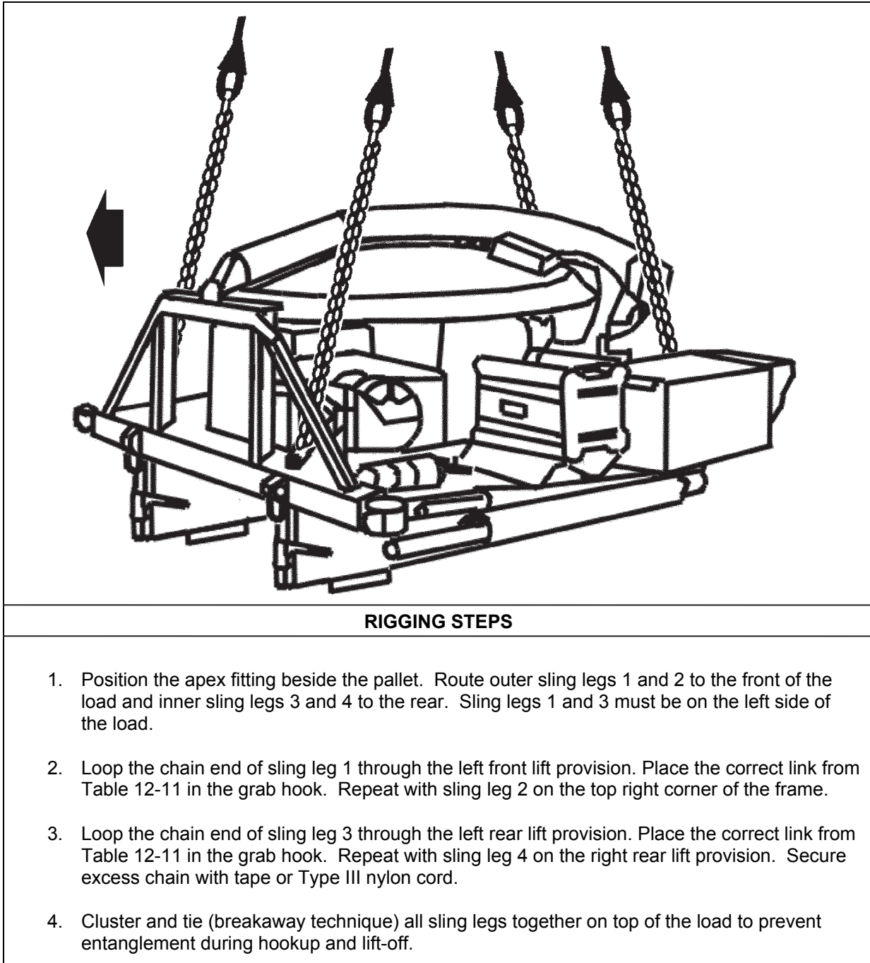
Figure 12-11. Secure Mobile Anti-Jam Reliable Tactical Terminal Pallet
