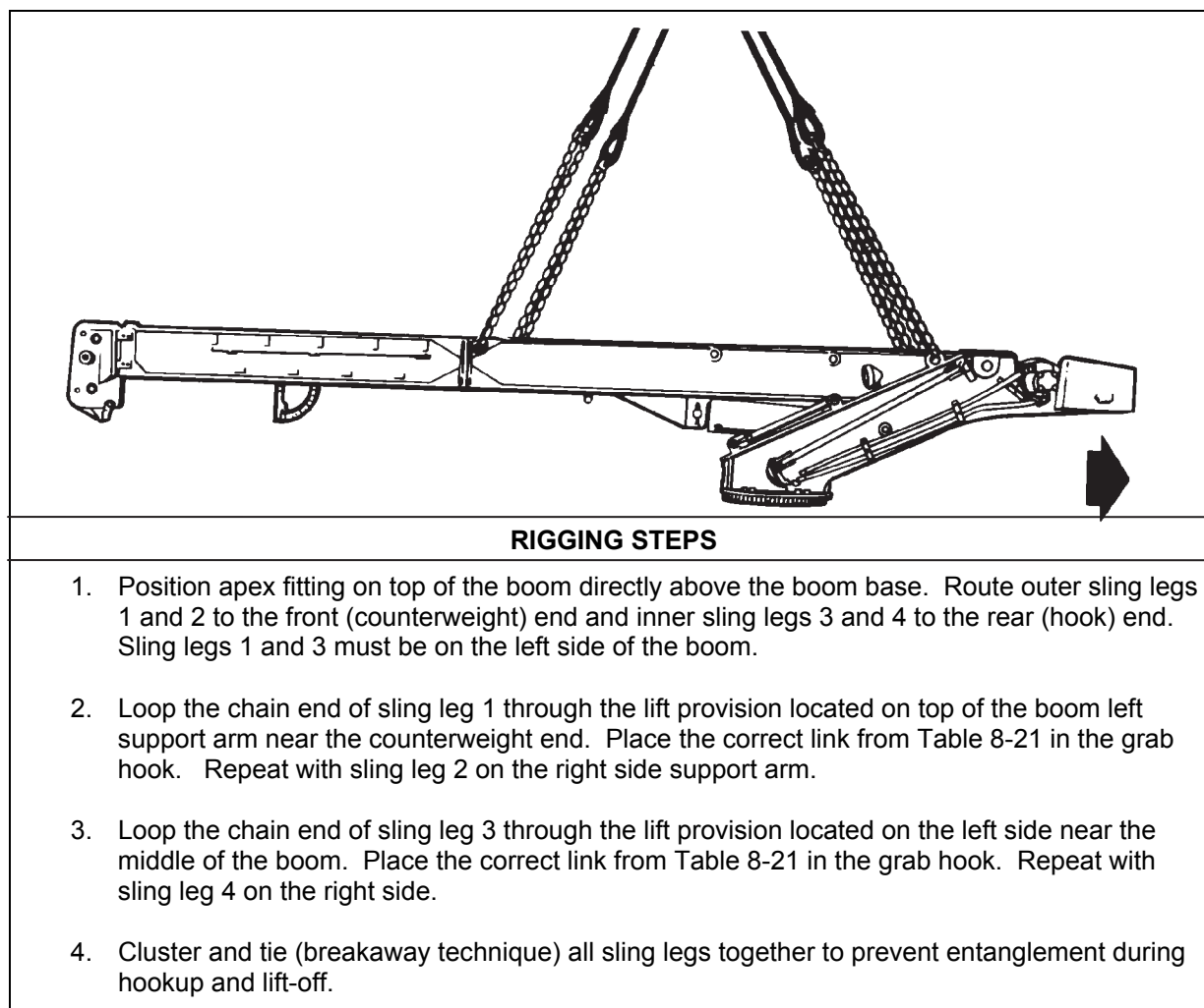
Figure 8-21. LRT-110, 7 1/2-Ton Crane Boom
