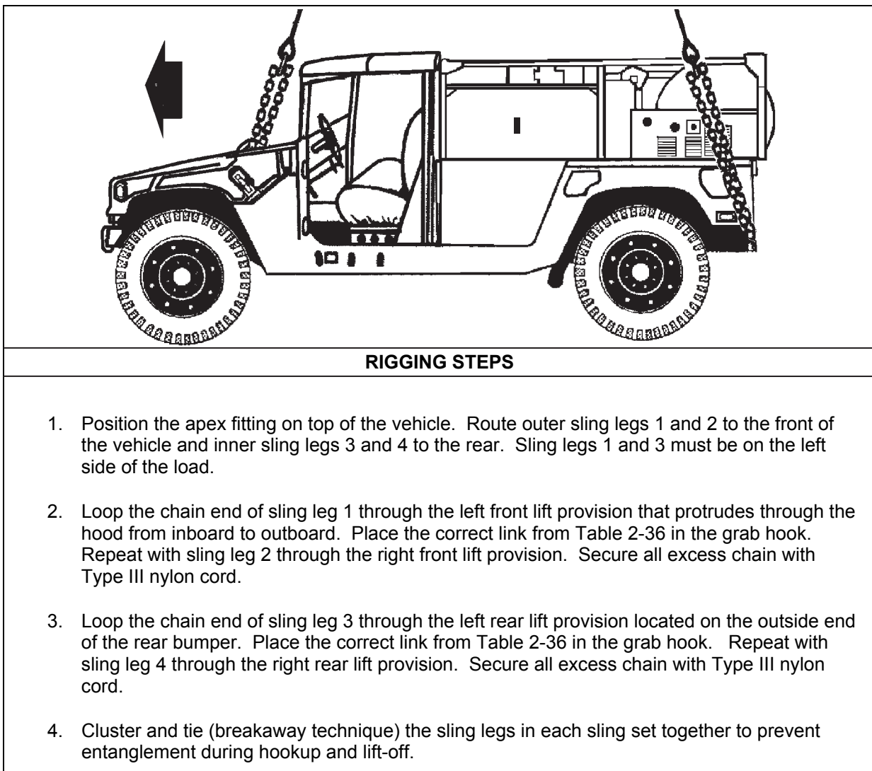
Figure 2-35. M1037 with Compressed Air-Foam System, Mobile
