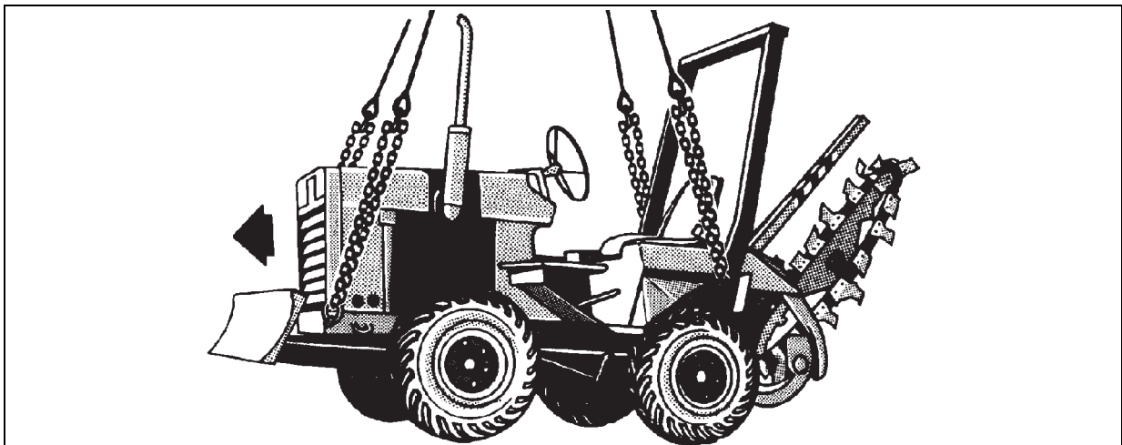
Figure 8-8. Ditching Machine
