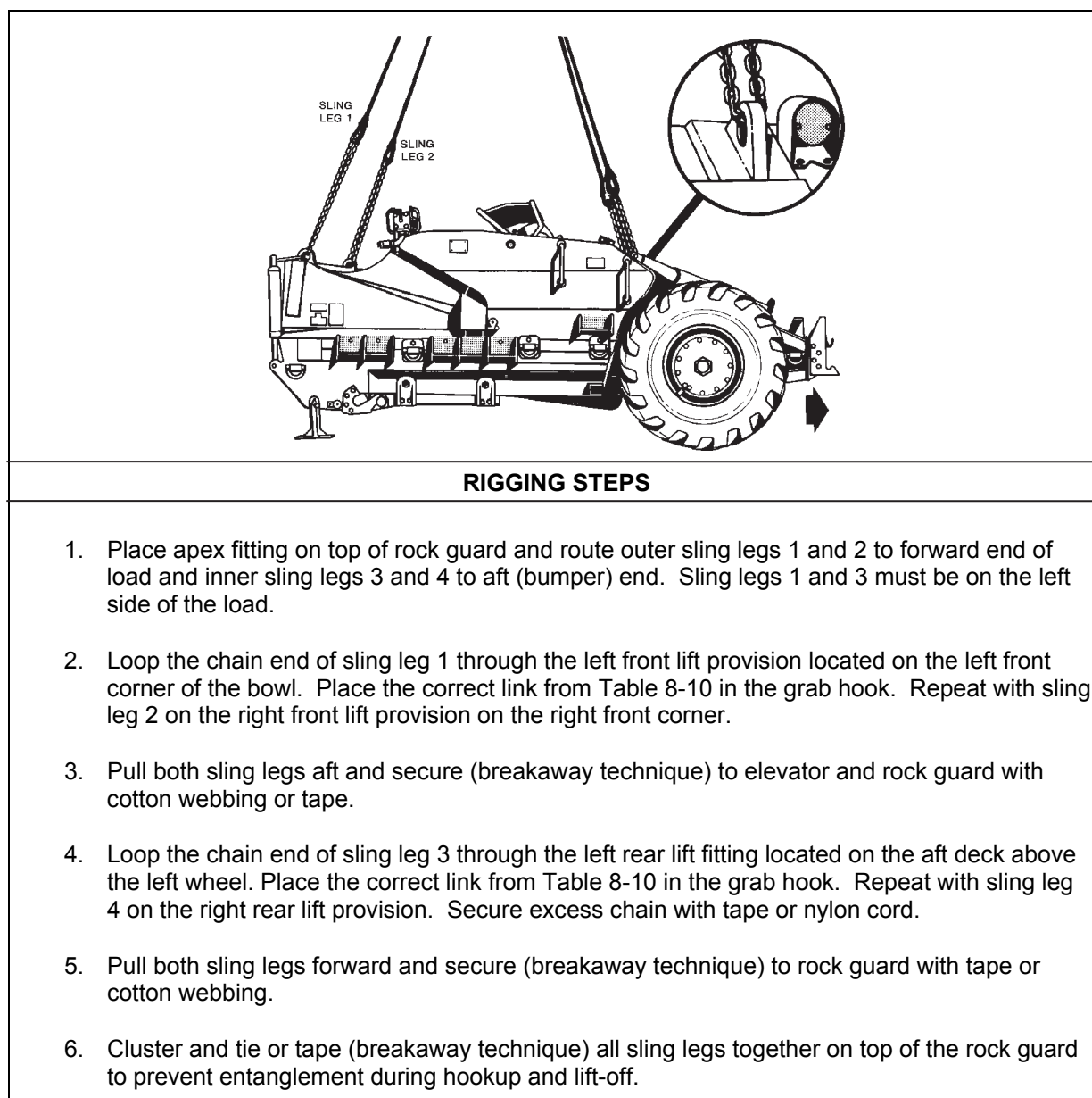
Figure 8-11. 613BS Elevating Scraper (Work Section)
