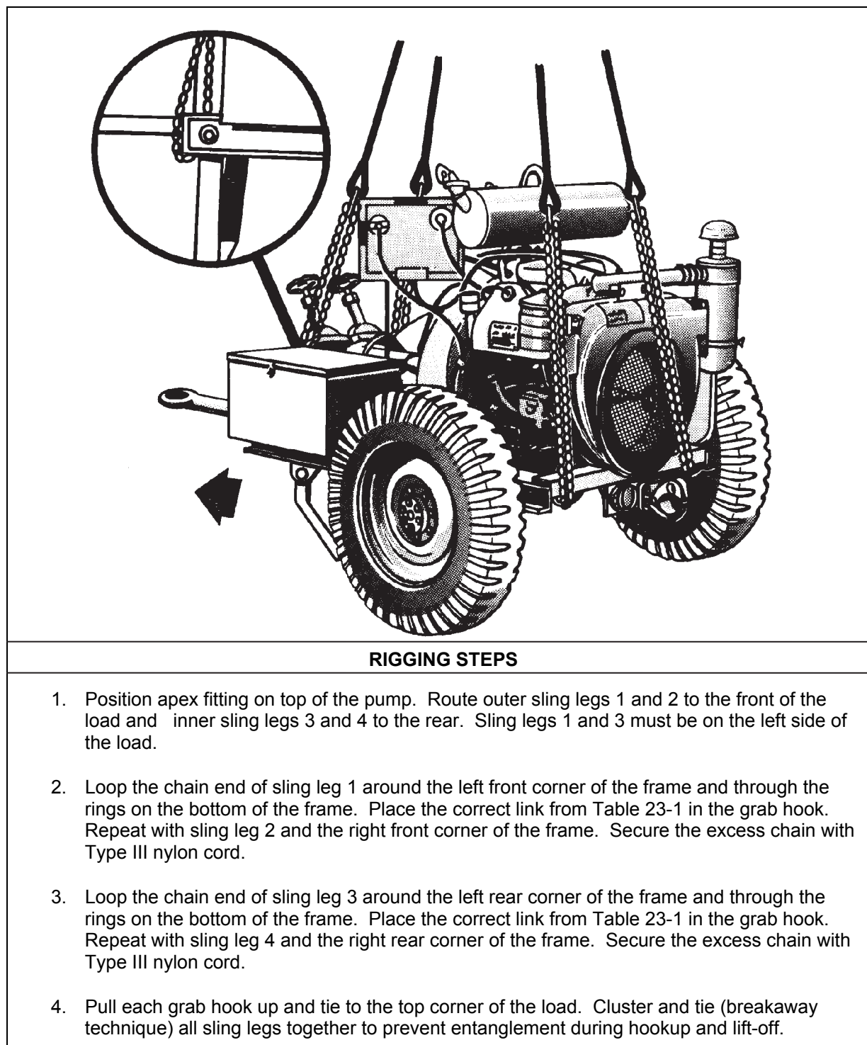
Figure 23-1. 350-GPM Pump Assembly
