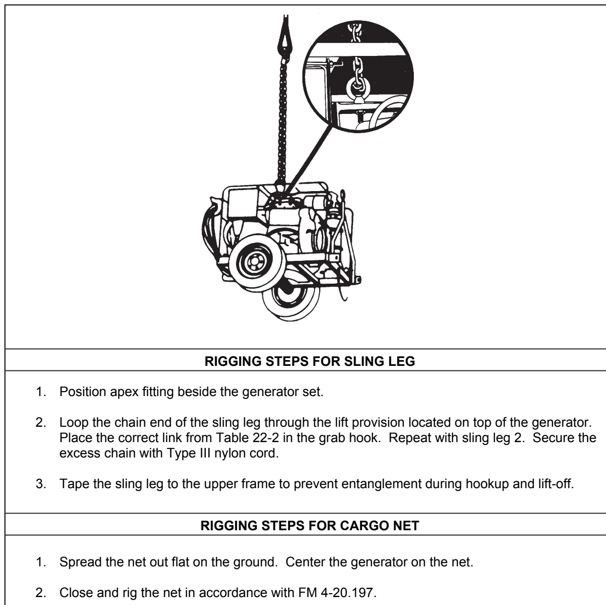
Figure 22-2. 7.5KW Generator Set
