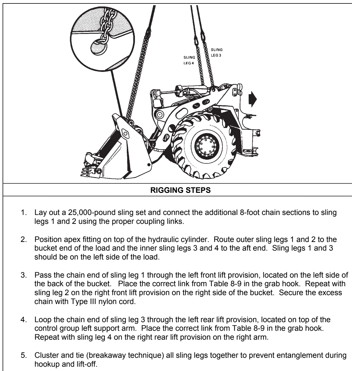
Figure 8-9. 950BS Scoop Loader (Work Section)
