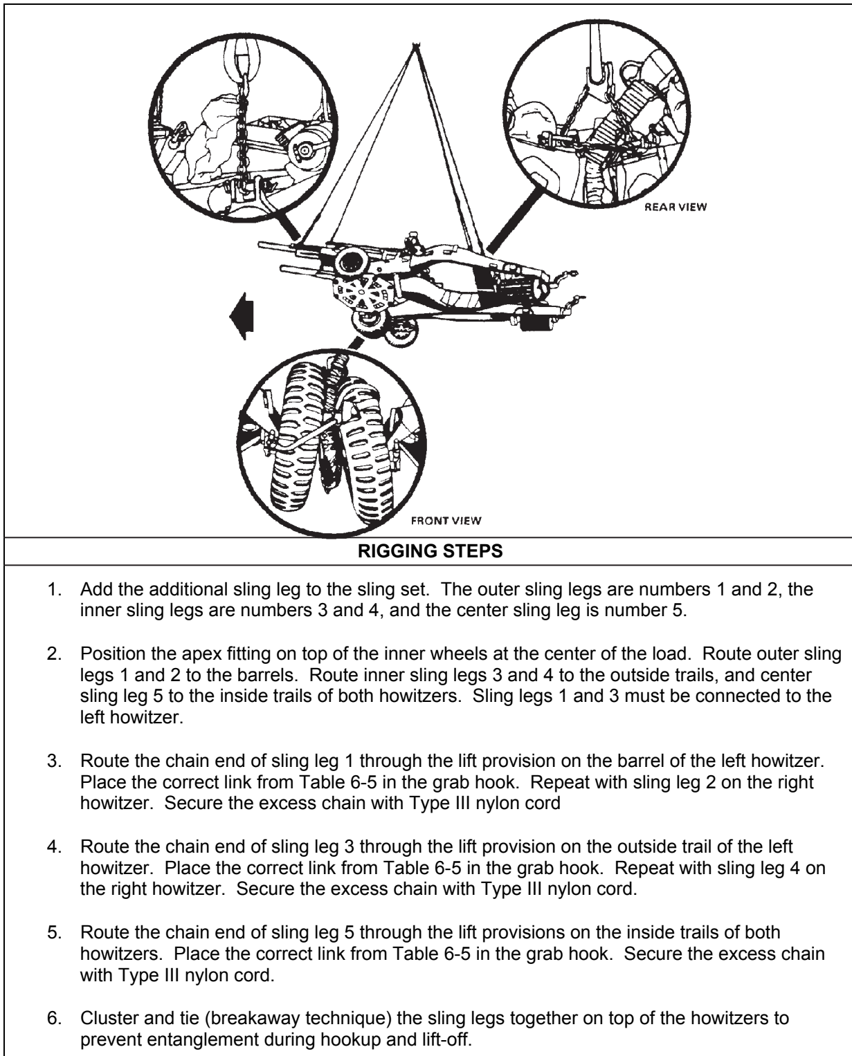
Figure 6-5. Two M102 105-MM Howitzers
