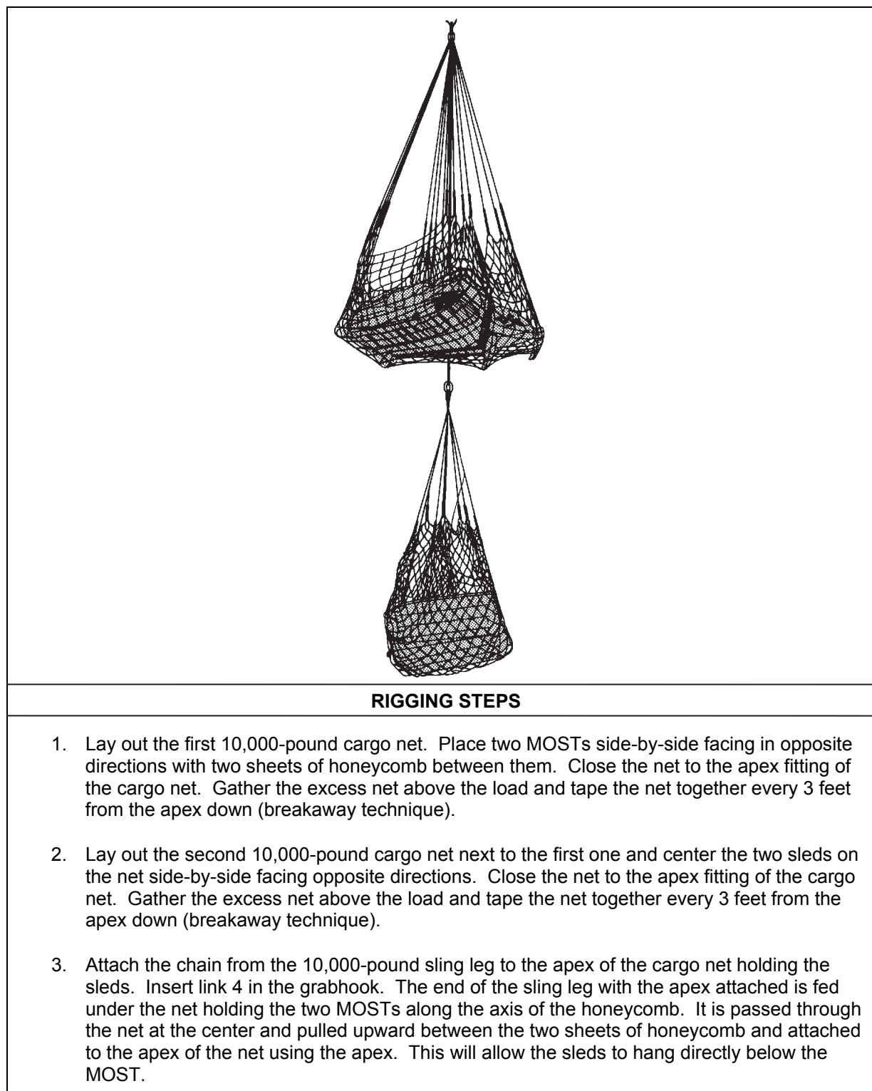
Figure 14-6. Two Mobile Oversnow Transport Snowmobiles with or without Two Sleds
