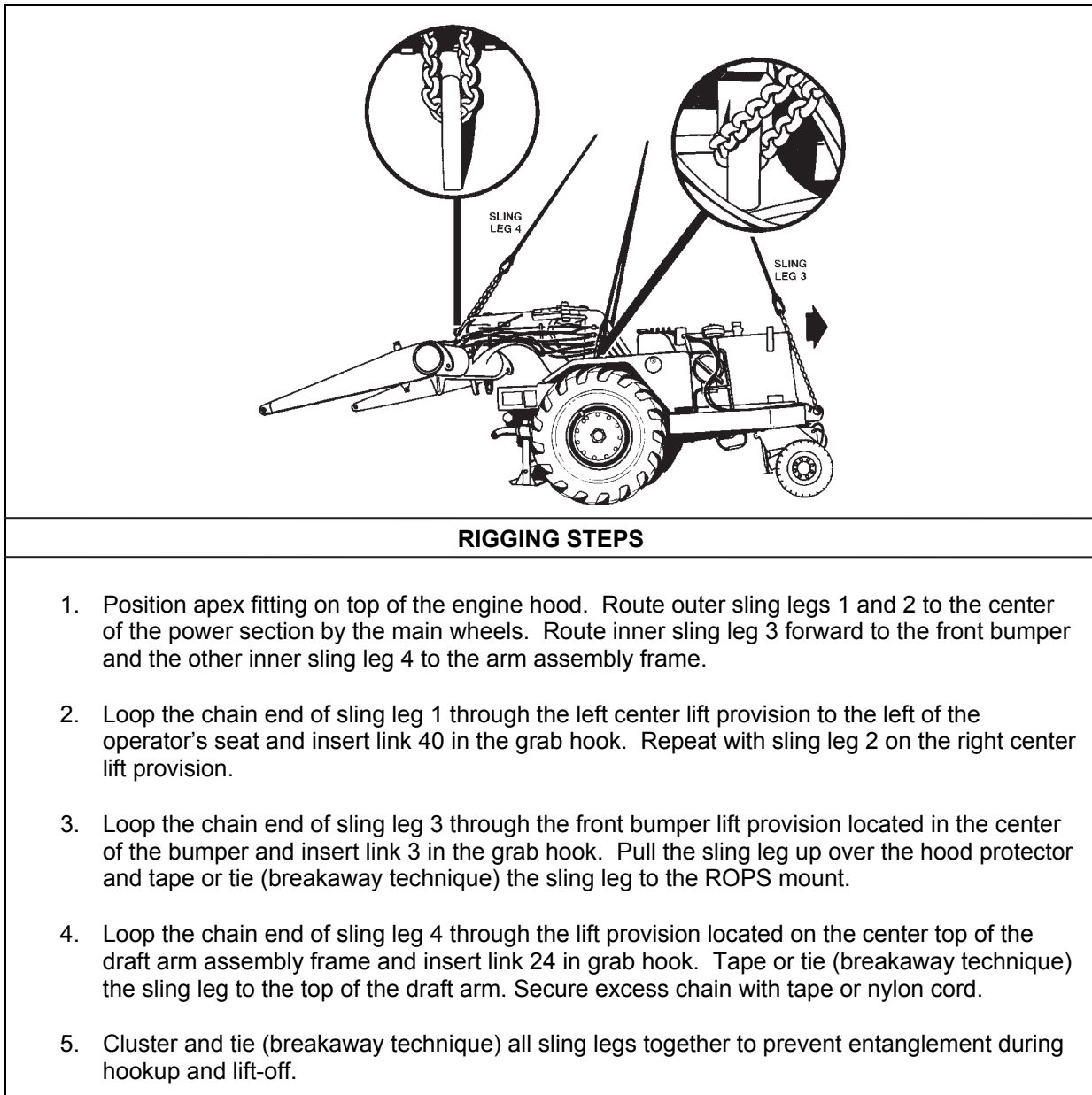
Figure 8-11. 613BS Elevating Scraper (Power Section)
