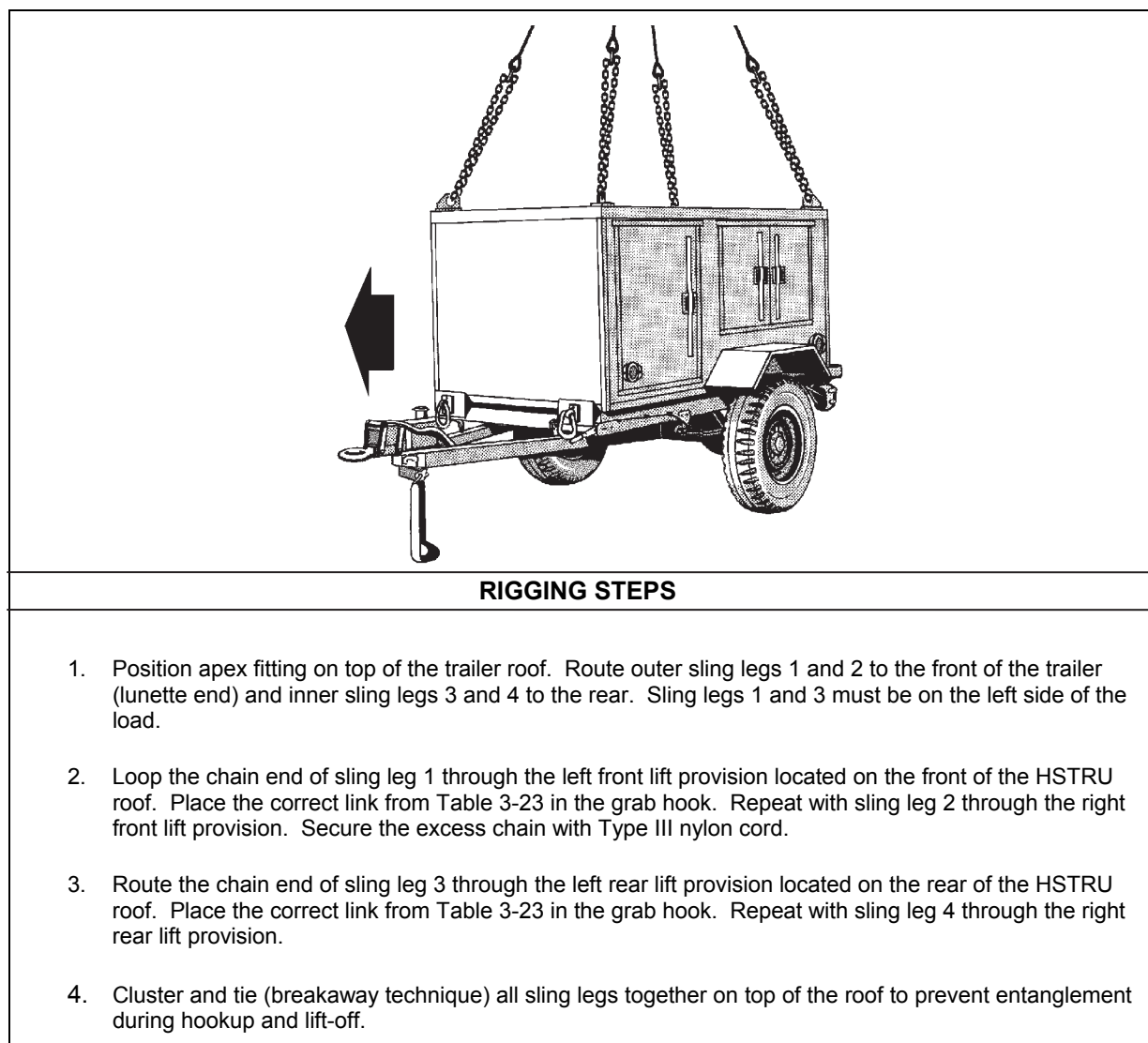
Figure 3-23. Hydraulic System Test and Repair Unit
