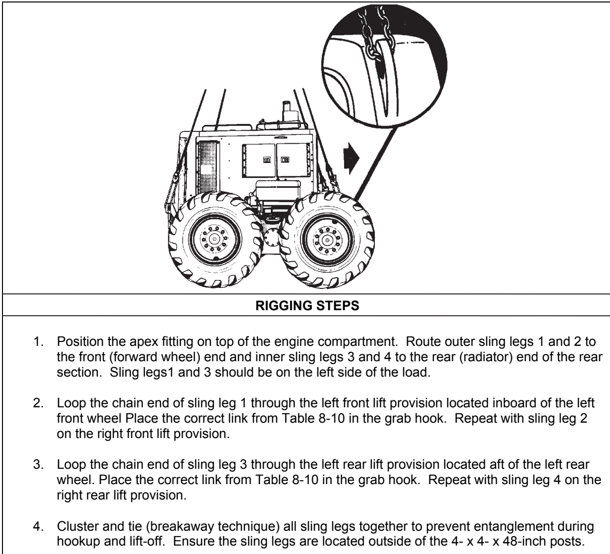
Figure 8-10. 130GS Grader (Rear Section)
