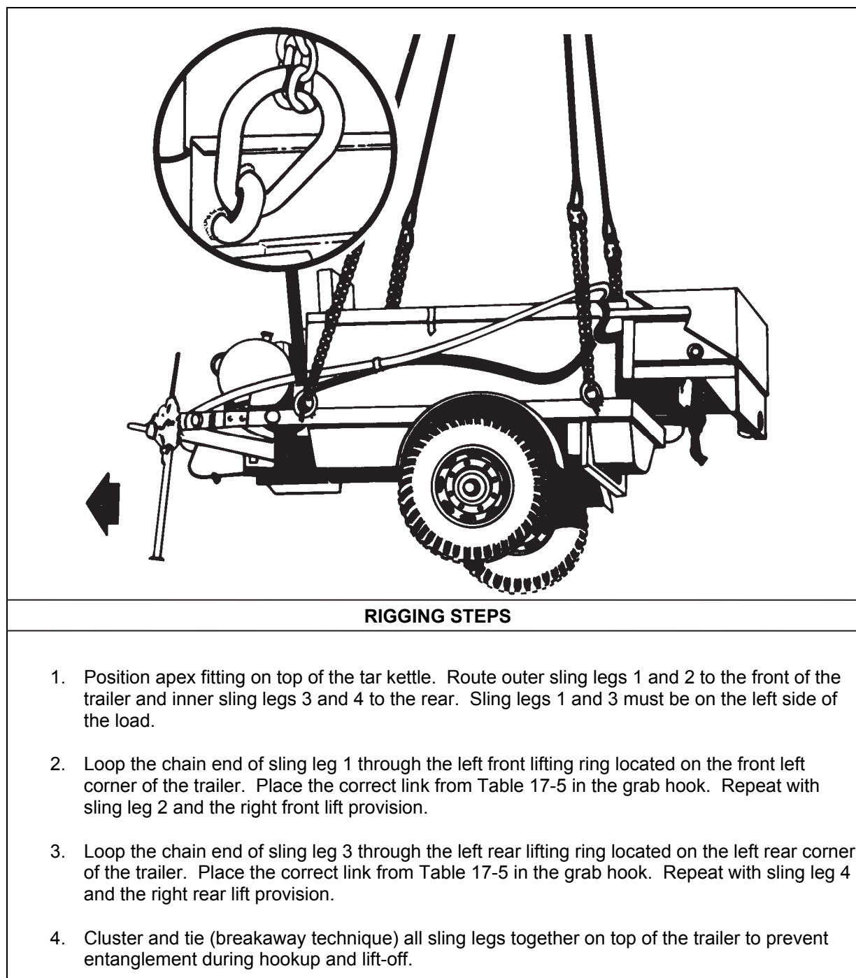
Figure 17-5. Tar Kettles
