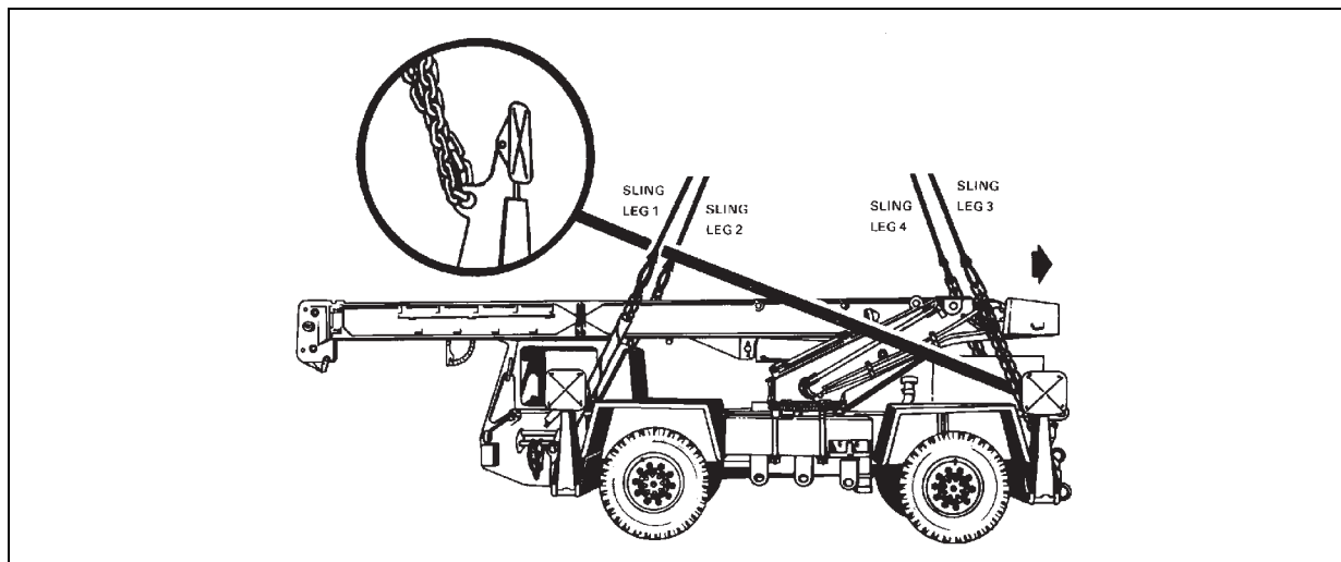
Figure 8-20. LRT-110, 7 1/2-Ton Crane
