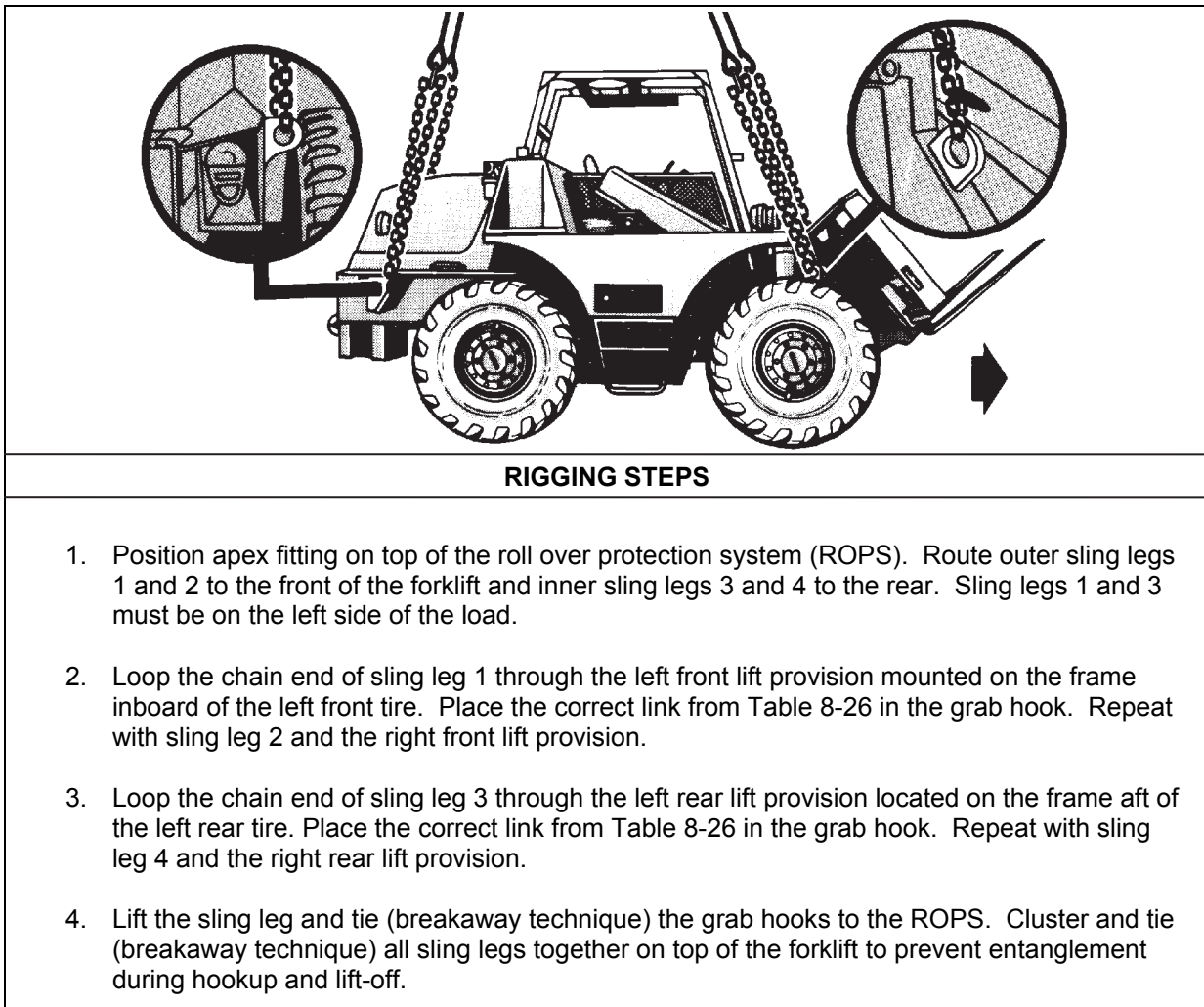
Figure 8-26. Truck, Forklift, MC-6000
