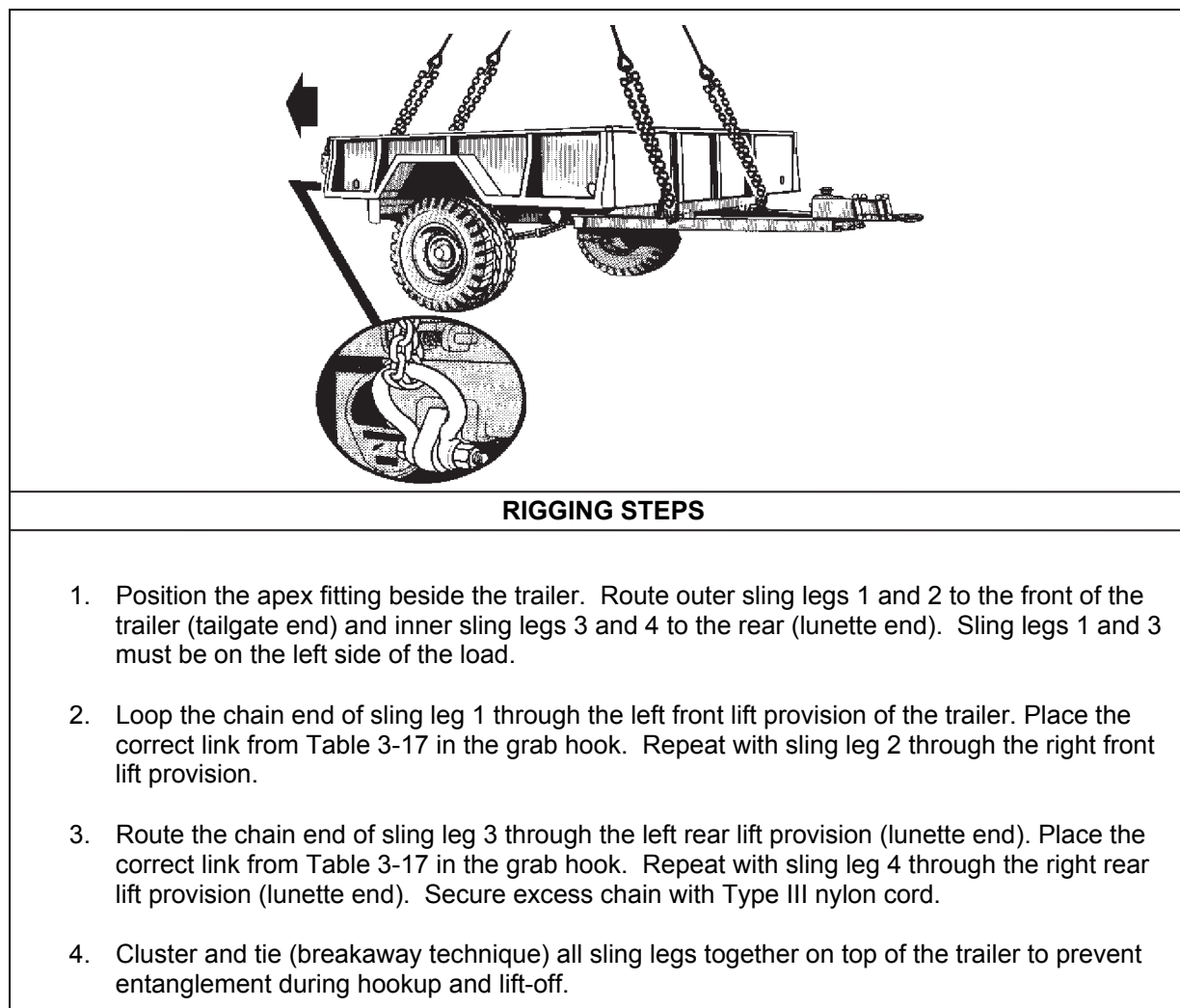
Figure 3-17. M105A3 Trailer
