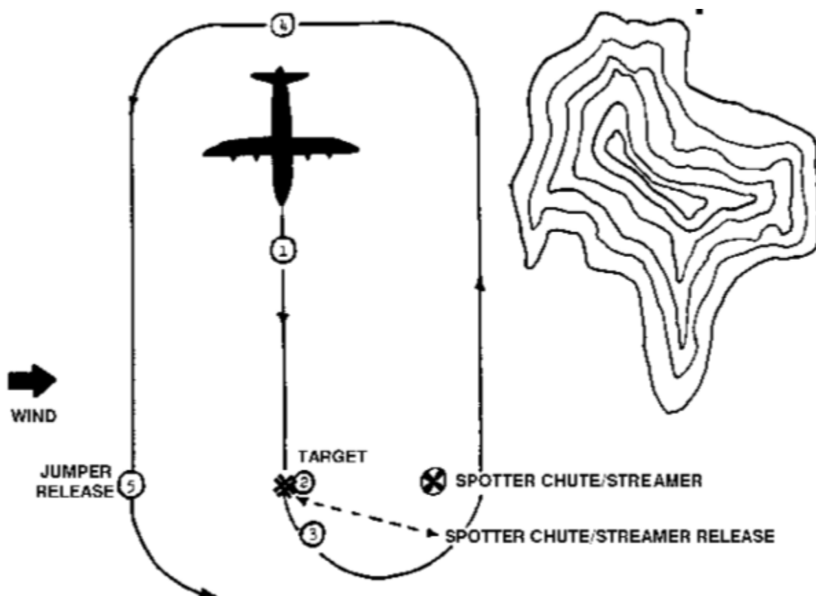
Figure A2.3. Crosswind Target Pattern.
