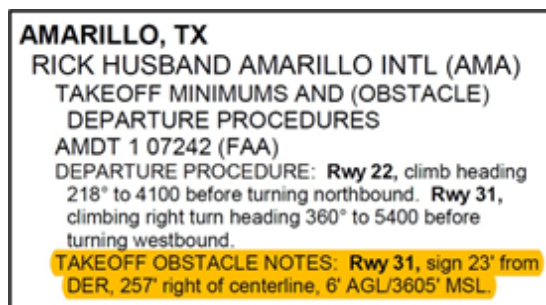
Figure 5.2. Low Close-in Obstacles.
