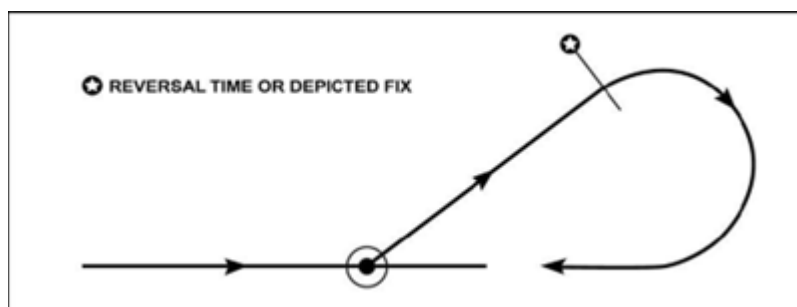
Figure 15.23. Base Turn or [NAS Only] Teardrop.
