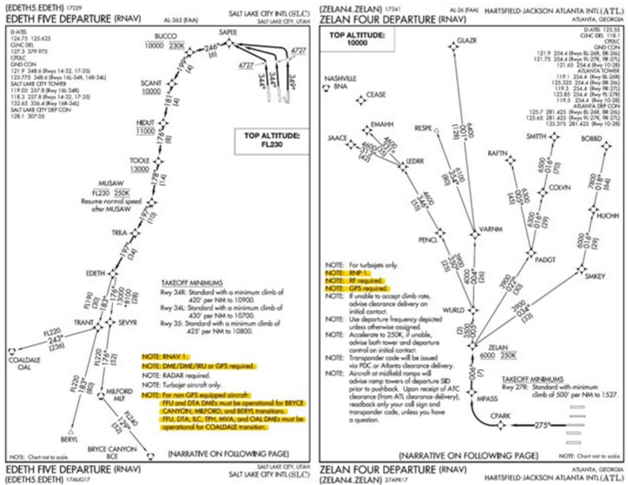
Figure 5.25. RNAV Departure Procedures.
