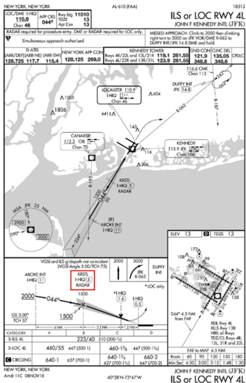
Figure 15.6. Radar Fix on Non-radar Approach.
