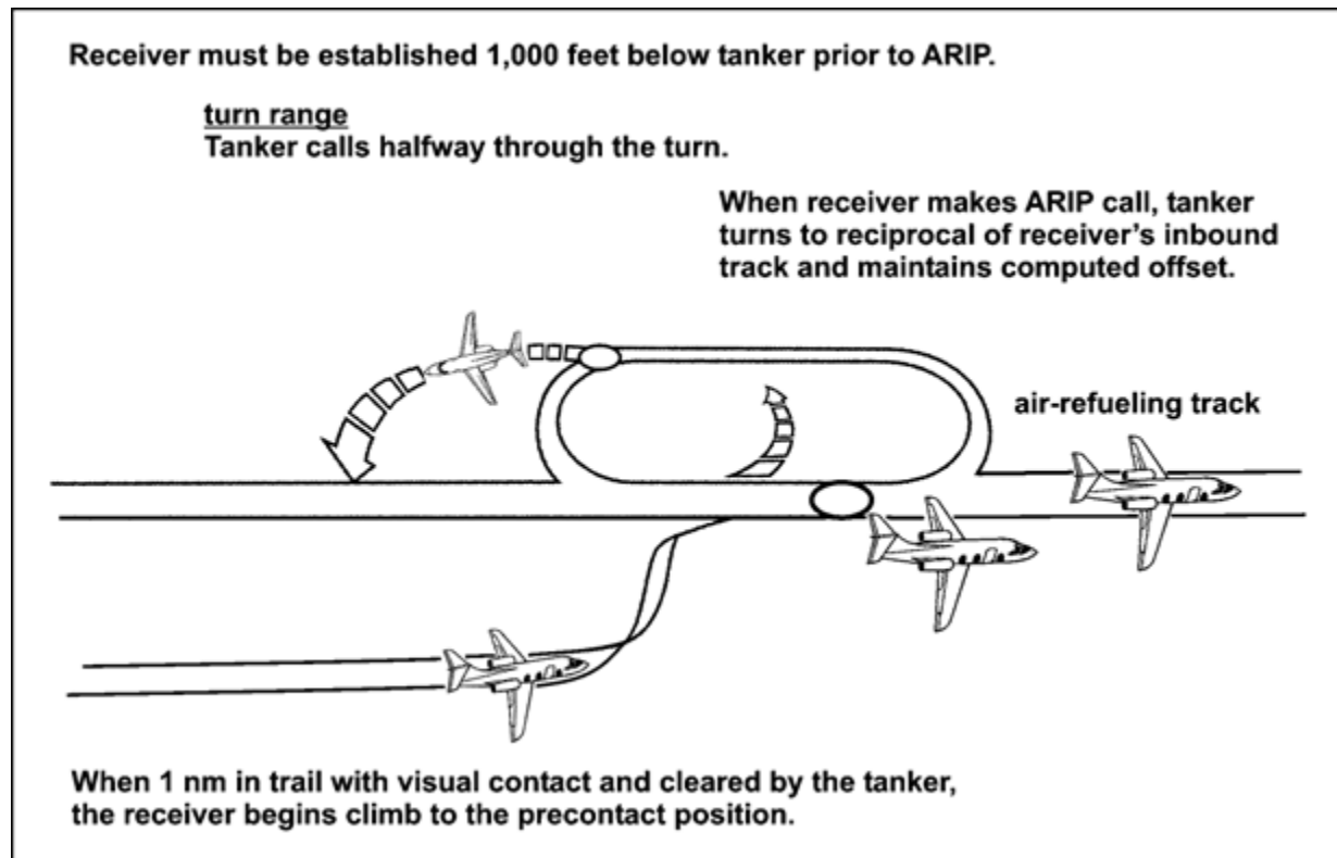
Figure 9.4. Air Refueling Rendezvous.
