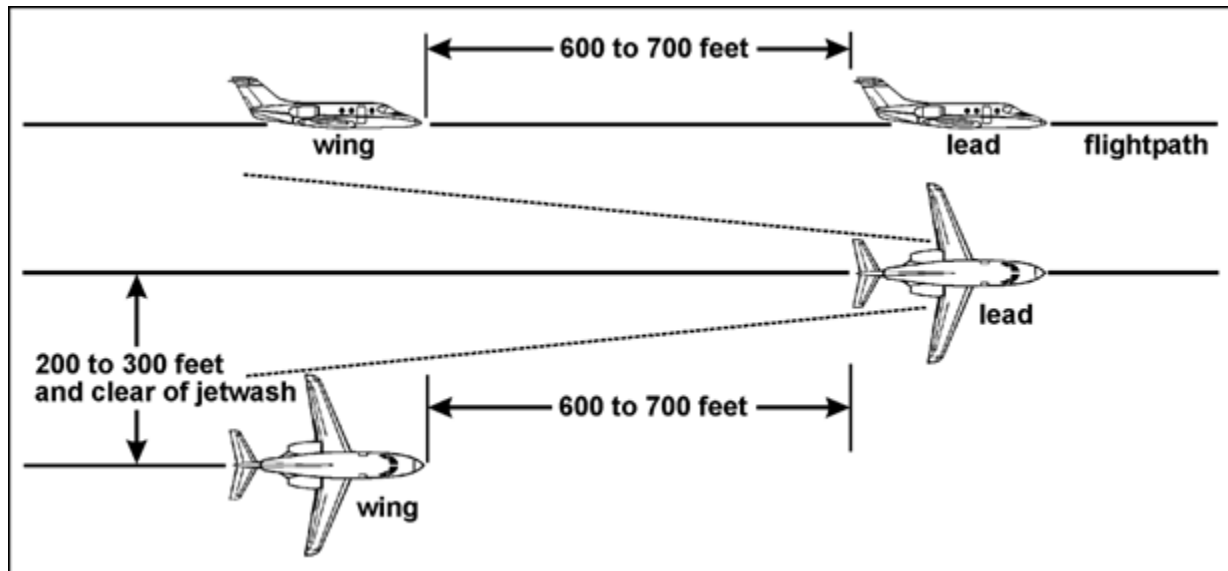
Figure 8.5. Visual Formation Position.
