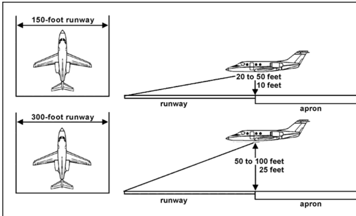
Figure 7.2. Visual Effect of a Wide Runway.
