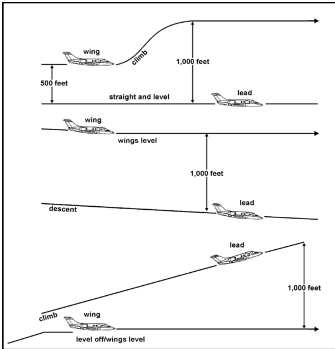
Figure 8.2. Cell Formation Lost Wingman.
