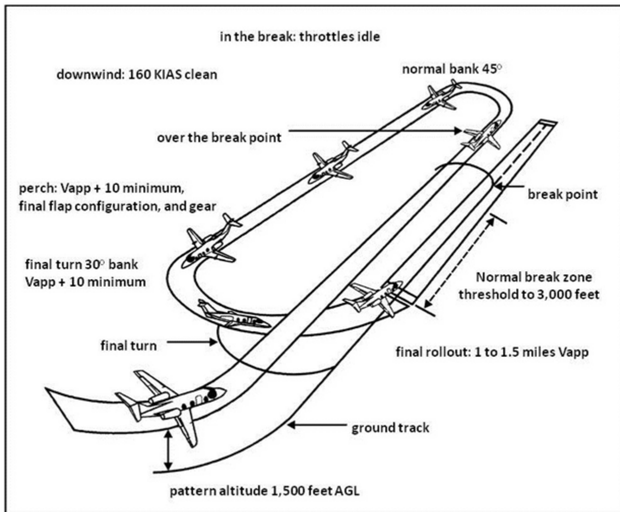
Figure 4.3. Tactical Pattern.
