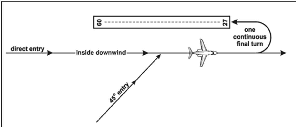
Figure 8.11. Formation Downwind Entry.
