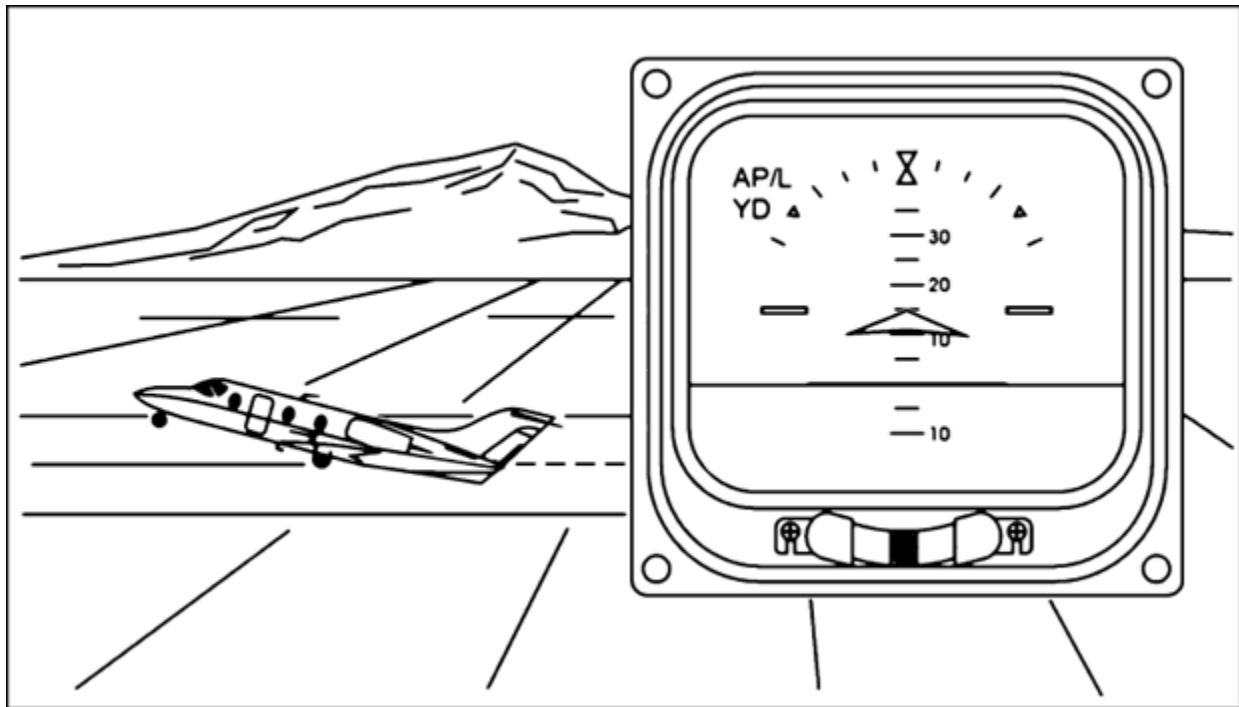
Figure 2.1. Takeoff Rotation.
