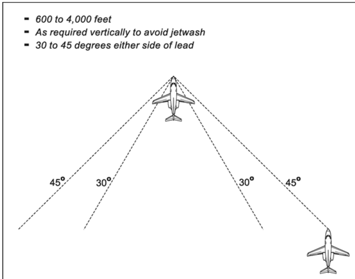
Figure 8.8. Offset Turns.
