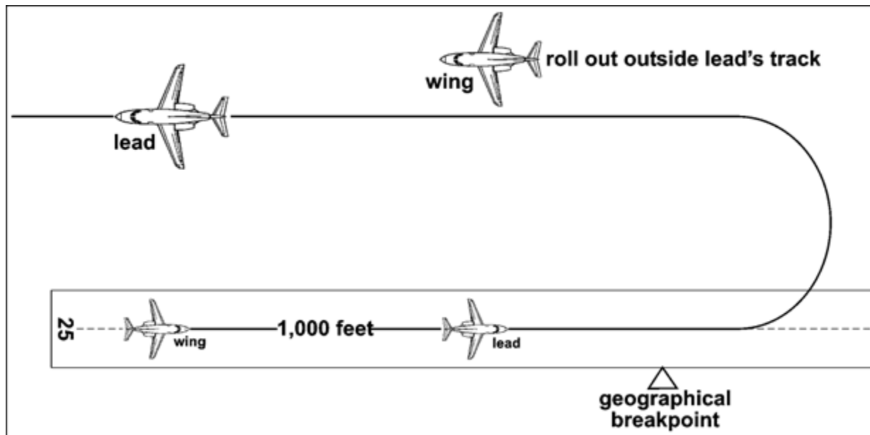
Figure 8.12. Pitchout Rollout Interval.
