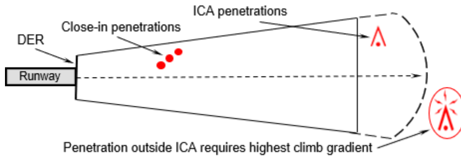
Figure 9.9. Case 9 Penetrations: All require >200 feet per NM climb gradient.
