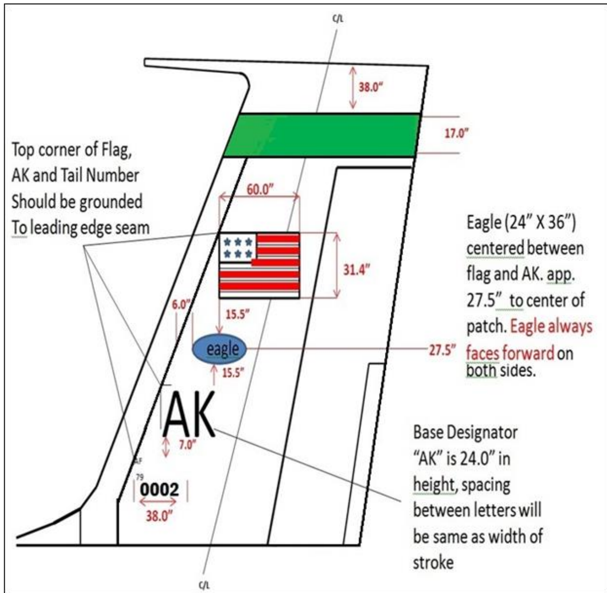
Figure A2.5. (Added-3WG) 3d Wing E-3 Aircraft Markings.
